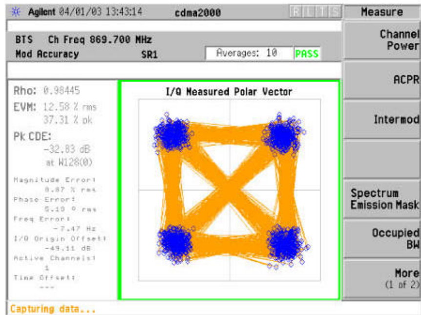
Channel 1013 – 869.7 MHz
