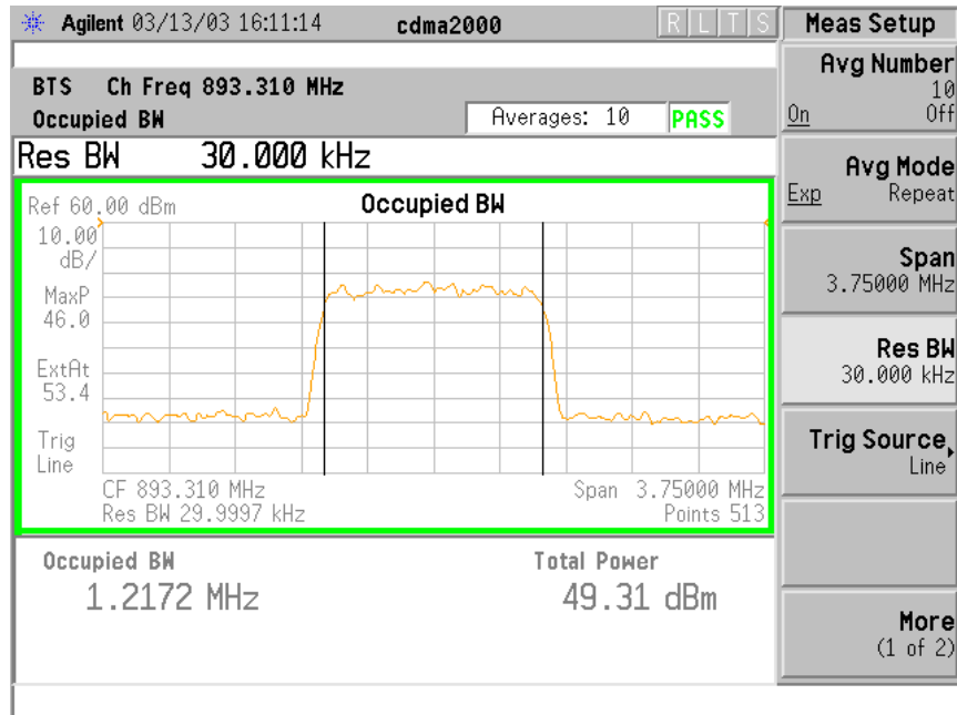
Channel 777 – 893.31 MHz
