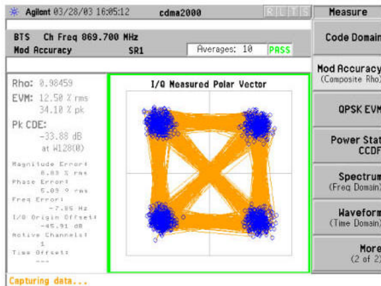
Channel 1013 – 869.7 MHz
