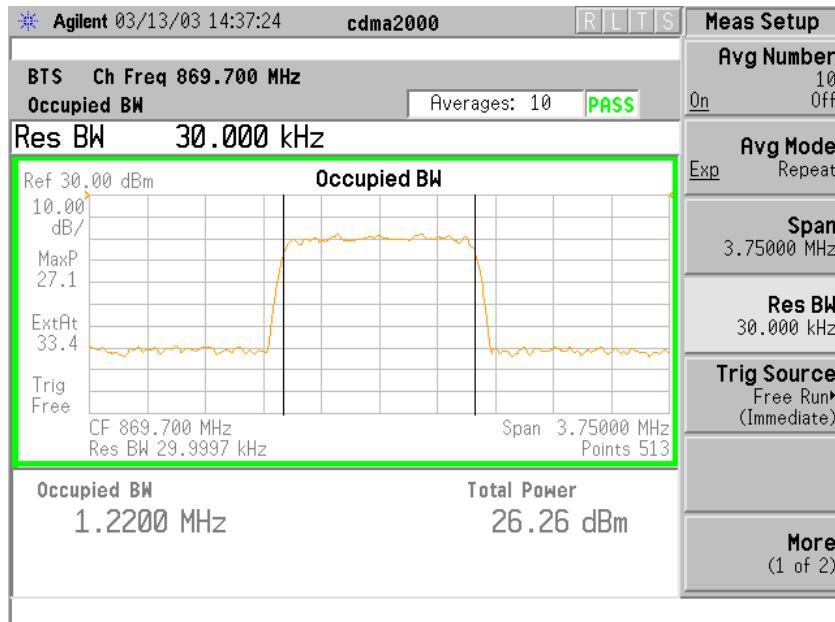
Channel 1013 – 869.7 MHz
