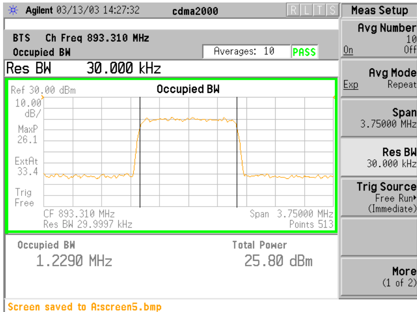
Channel 777 – 893.31 MHz
