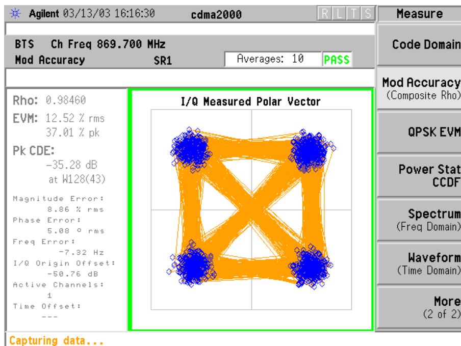
Channel 1013 – 869.7 MHz
