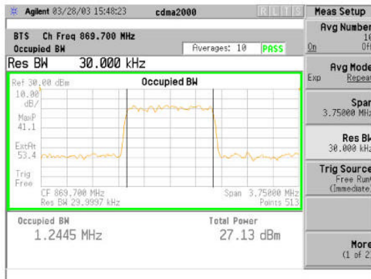
Channel 1013 – 869.7 MHz
