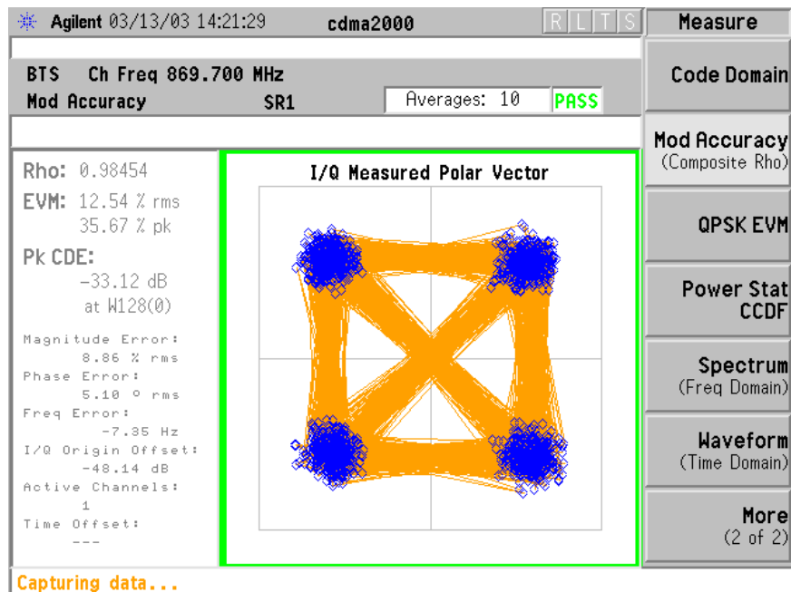
Channel 1013 – 869.7 MHz
