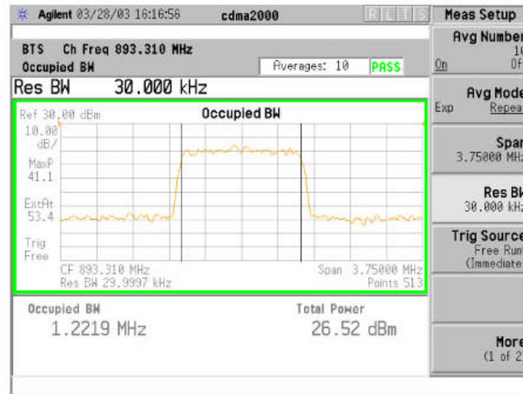
Channel 777 – 893.31 MHz
