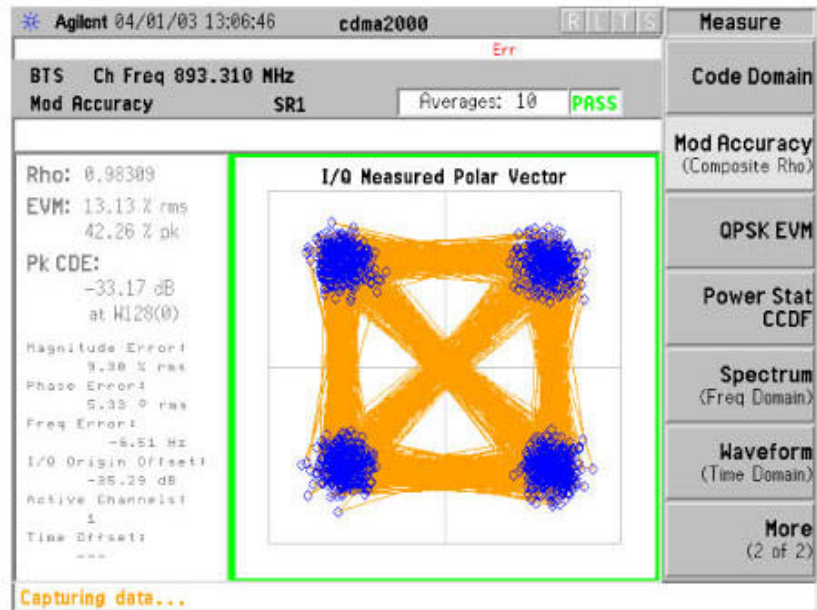
Channel 777 – 893.31 MHz
