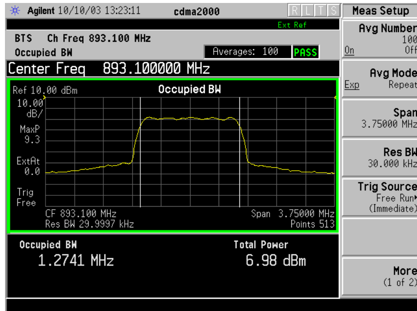
Channel 770 – 893.1 MHz
