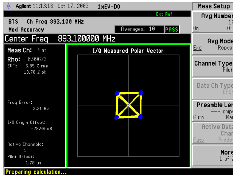
Channel 770 – 893.1 MHz
