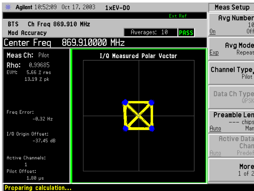
Channel 1020 – 869.91 MHz
