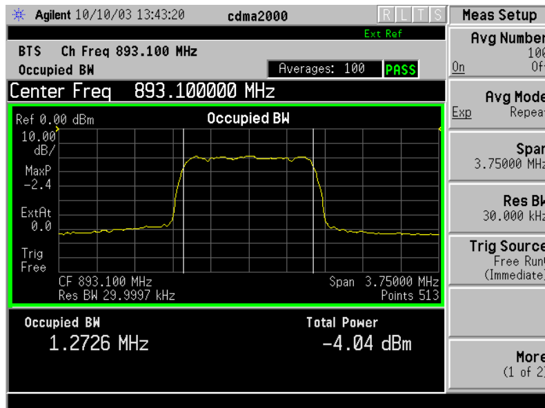
Channel 770 – 893.1 MHz
