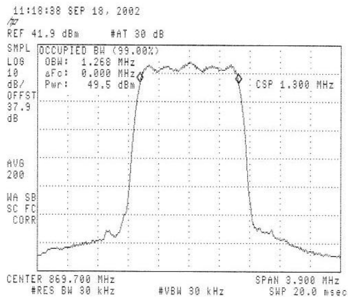
Channel 1013 – 869.7 MHz
