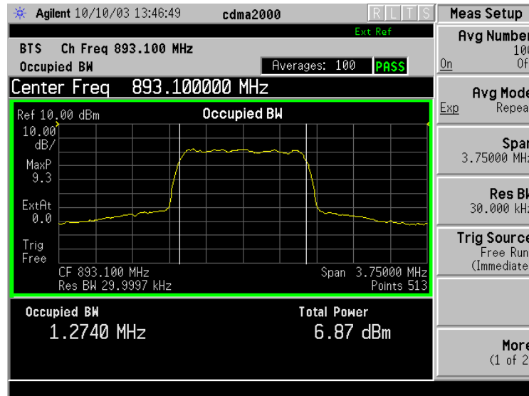
Channel 770 – 893.1 MHz
