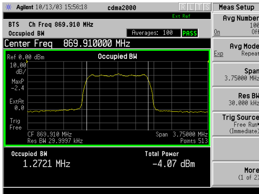
Channel 1020 – 869.91 MHz
