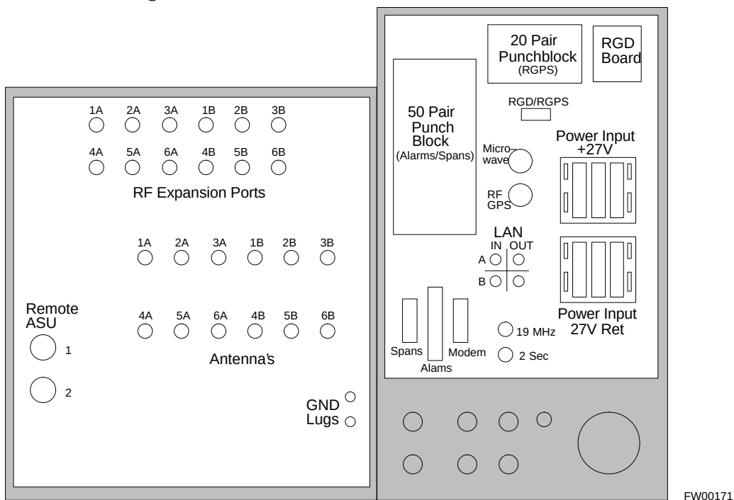
Figure 1-7: SC 4812ET I/O Plate Diagram
