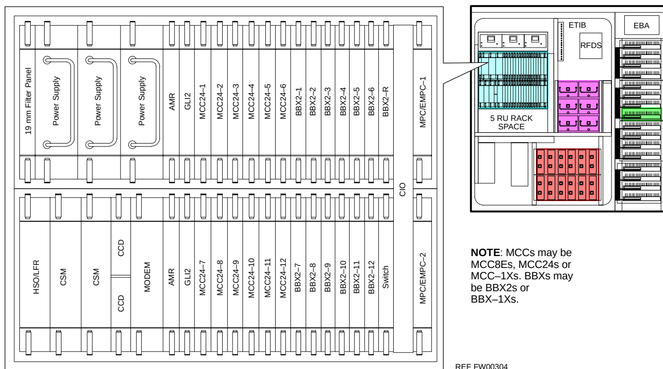
Figure 1-5: SC 4812ET C-CCP Shelf
