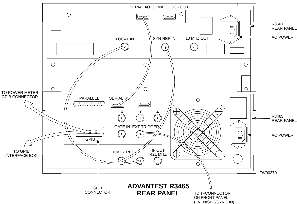
Figure F-3: Cable Connections for Test Set without 10 MHz Rubidium Standard
