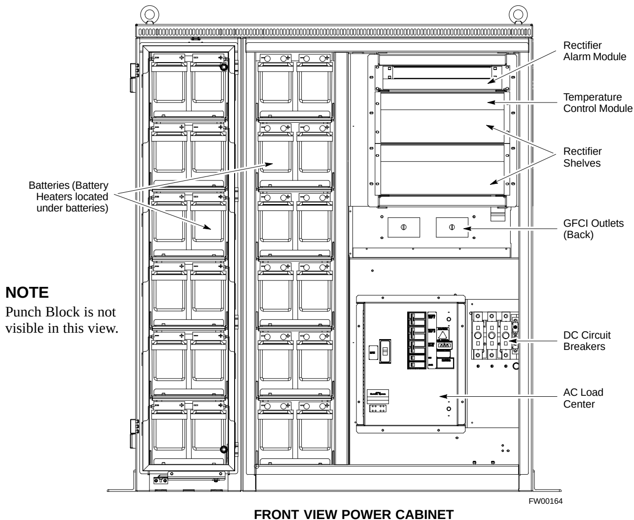
Figure 1-11: Power Cabinet with Batteries Installed (Doors Removed for Clarity)
