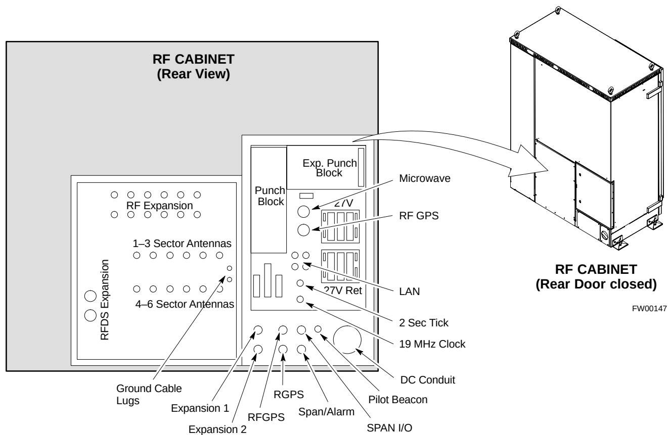
Figure 1-6: SC 4812ET Intercabinet I/O Detail (Rear View)
