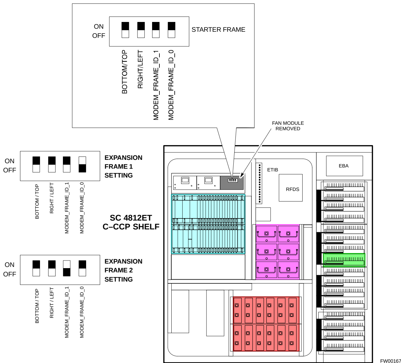
Figure 2-1: Backplane DIP Switch Settings
