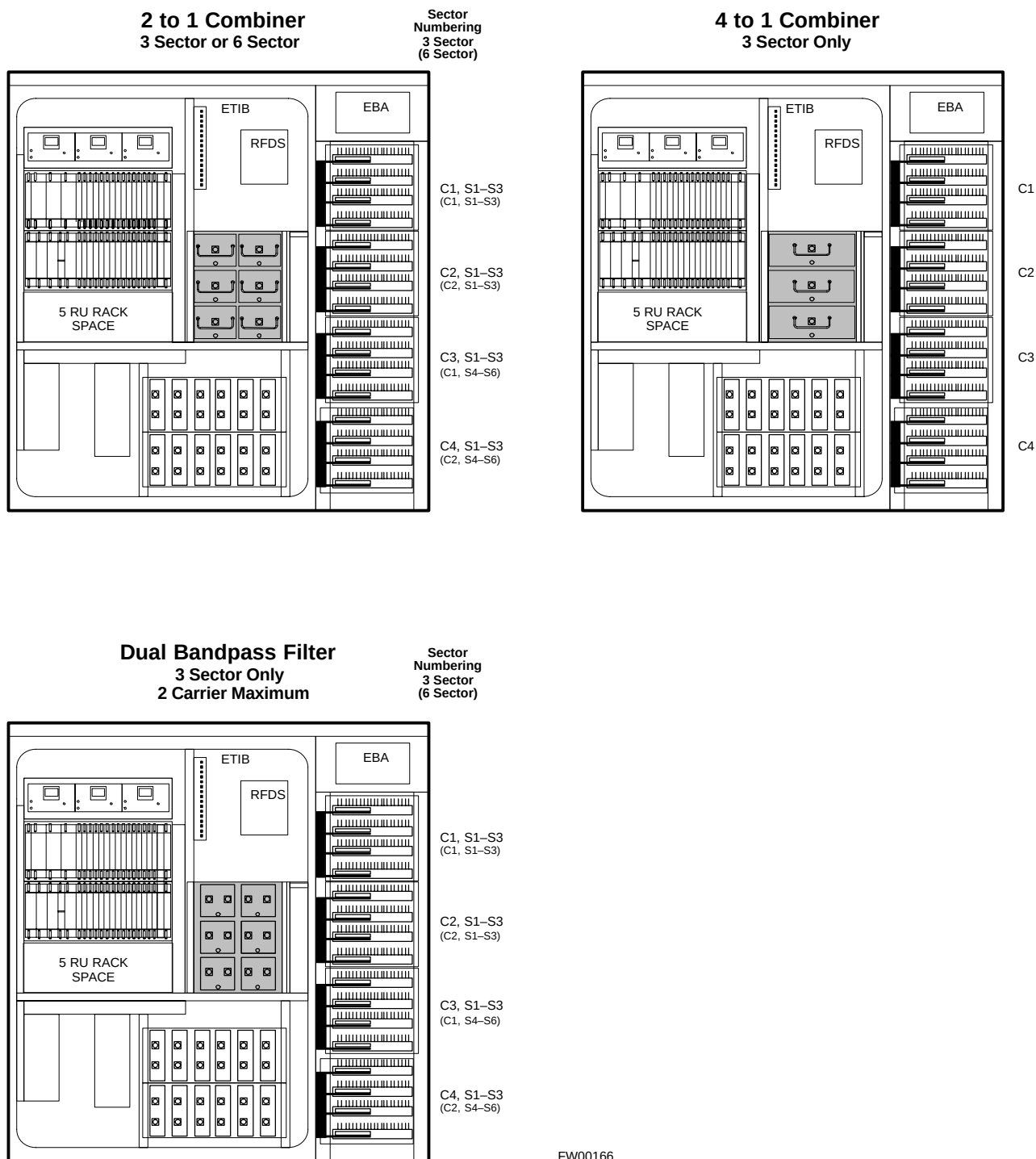
Figure 1-9: SC4812ET LPA Configuration with Combiners/Filters
