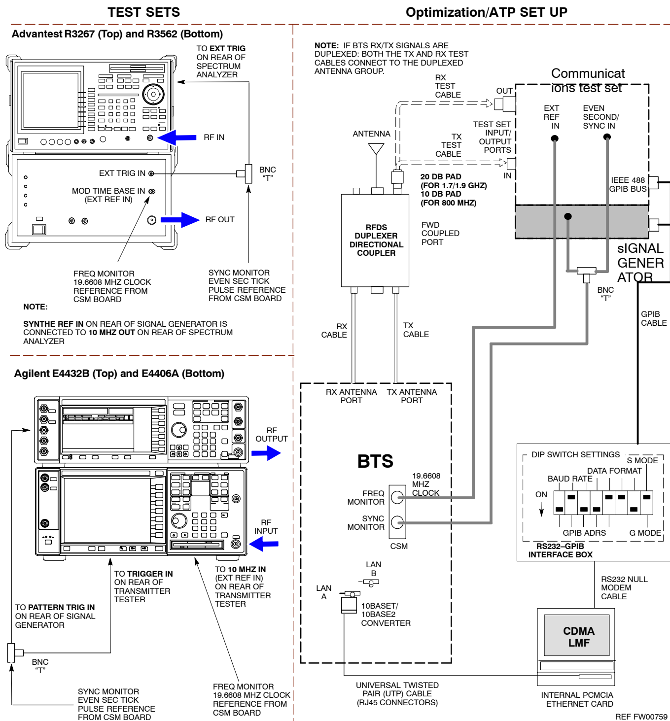
Figure H-10: IS-95 A/B/C Optimization/ATP Test Setup Using RFDS
