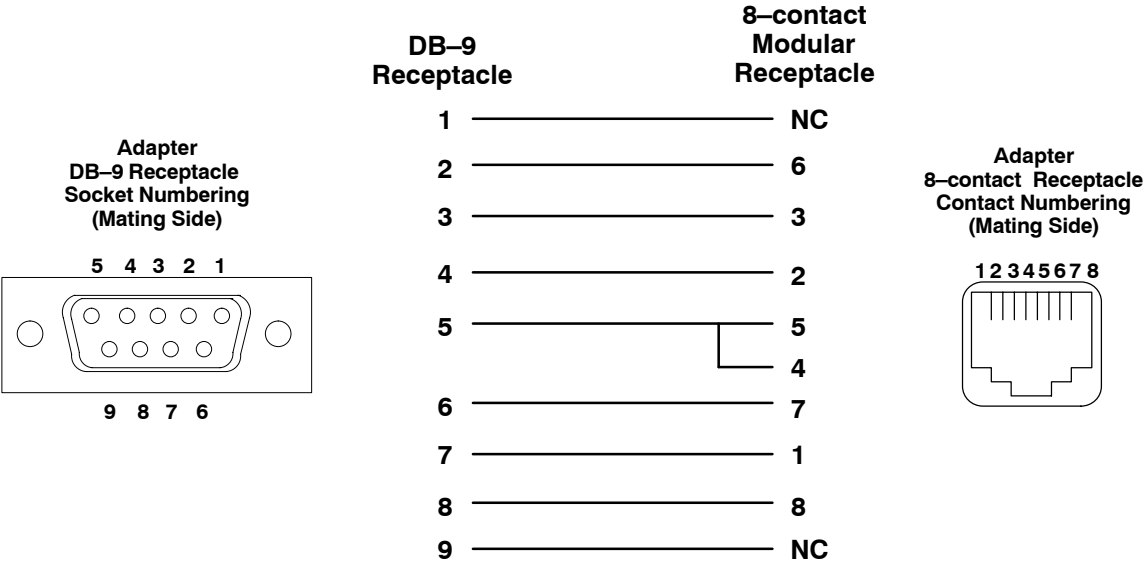
Figure J-2: Wiring Diagram, DB-9 Plug-to-8-contact Modular Plug Adapter
