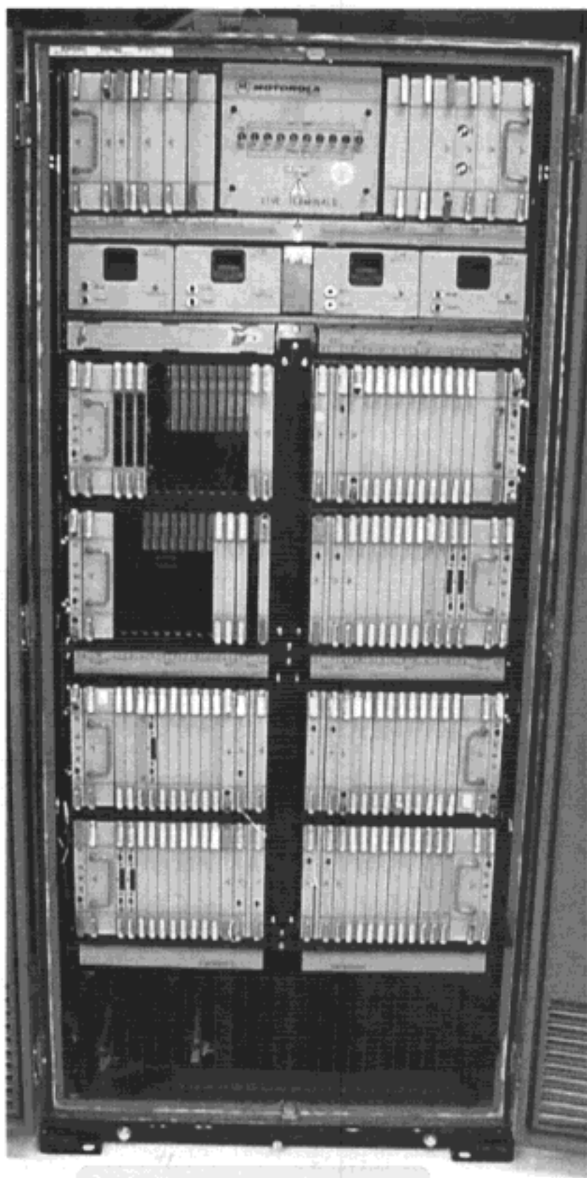
IHET5YE1 SC9600 Mixed Mode/Multiple Carrier Front View-Door Open
