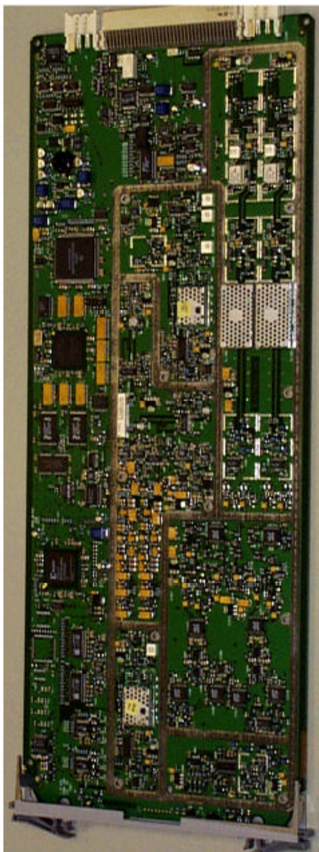
IHET5YP1 SC4812T 800 MHz BBX2 without Cover
