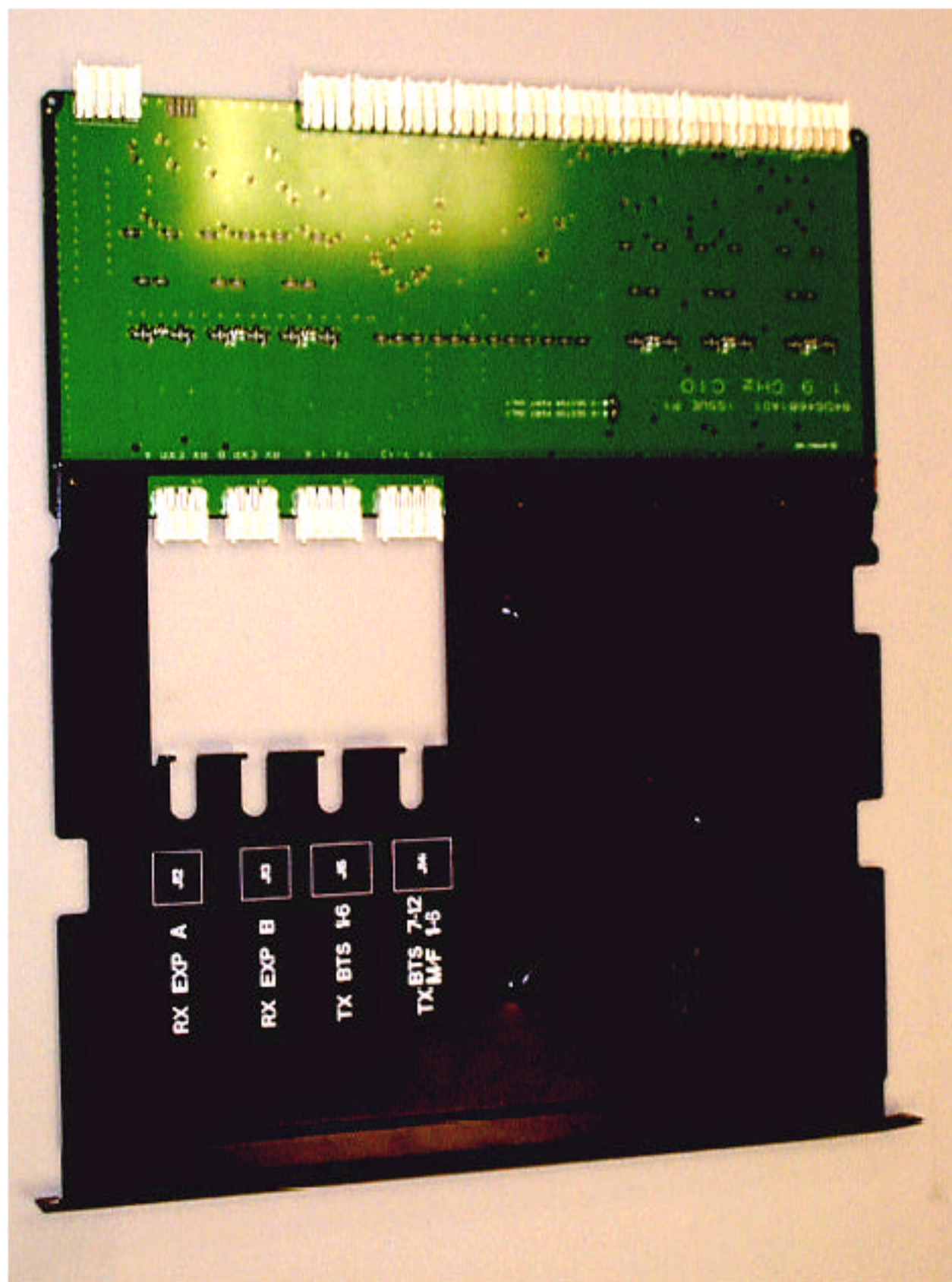
IHET5YP1 SC4812T 800 MHz CIO Front
