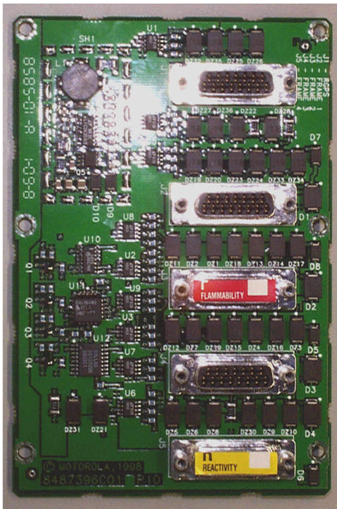
IHET5YP1 SC4812T 800 MHz RGD Front
