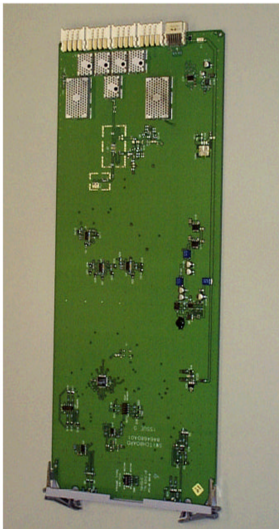
IHET5YP1 SC4812T 800 MHz Switch Card Front
