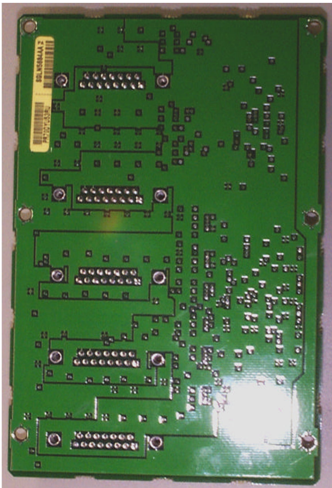
IHET5YP1 SC4812T 800 MHz RGD Back
