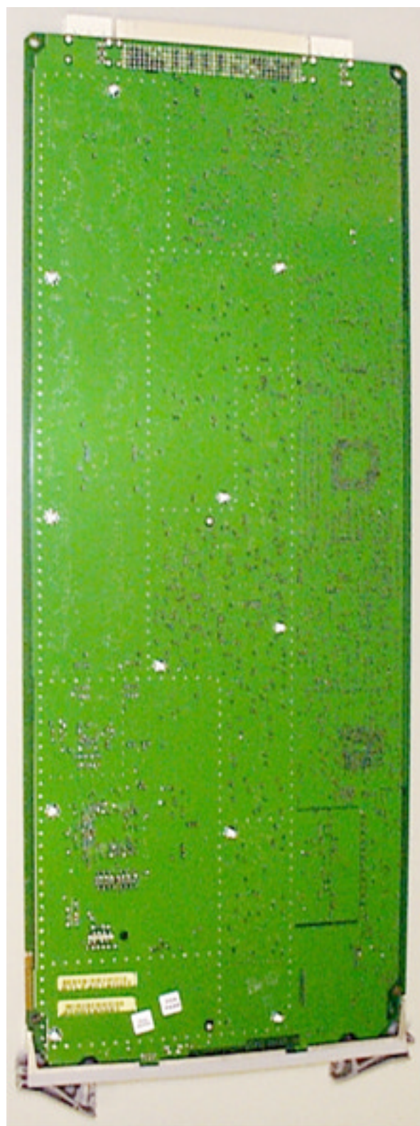
IHET5YP1 SC4812T 800 MHz DBPBBX Back
