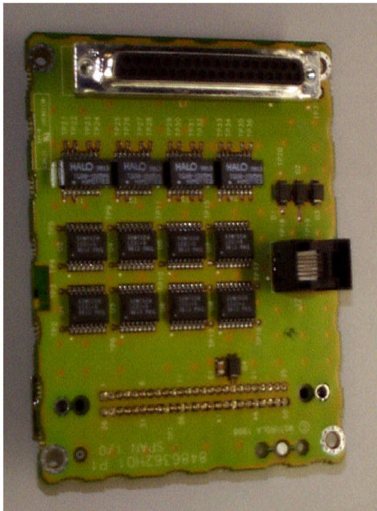
IHET5YP1 SC4812T 800 MHz Span I/O Back
