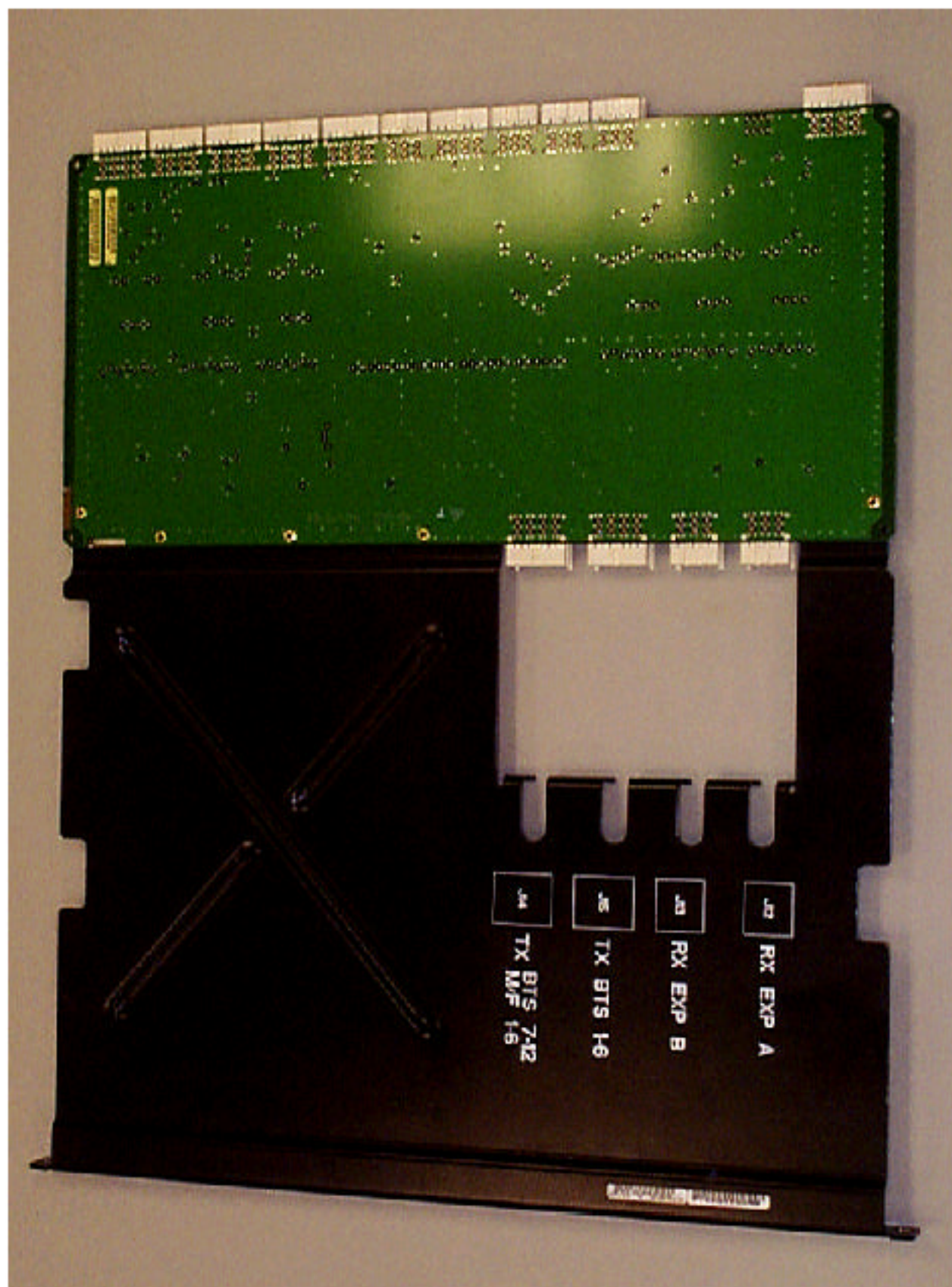
IHET5YP1 SC4812T 800 MHz CIO Back
