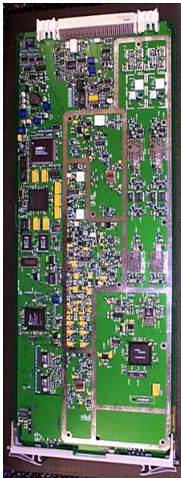
IHET5YP1 SC4812T 800 MHz DBPBBX Front without Cover
