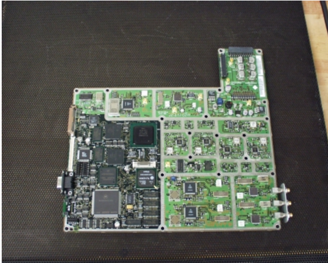
IHET6BV1 HorizonMacro1900 Transceiver Board Rear View
