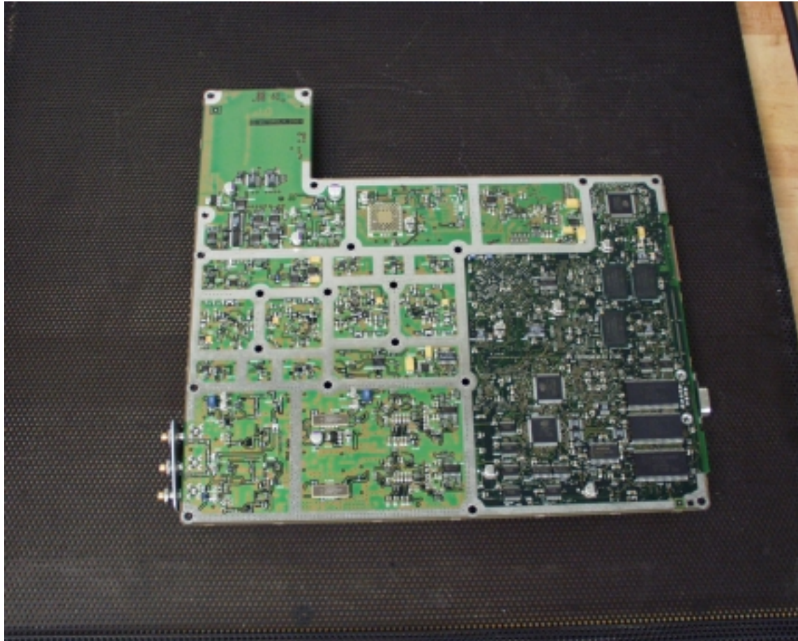
IHET6BV1 HorizonMacro1900 Transceiver Board Front View
