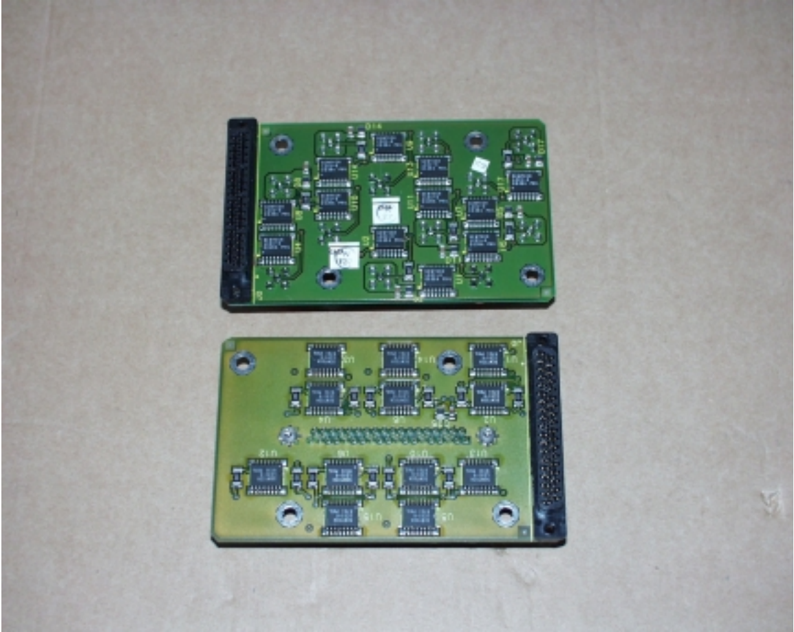
IHET6BV1 HorizonMacro1900 Line Interface Cards Rear View
