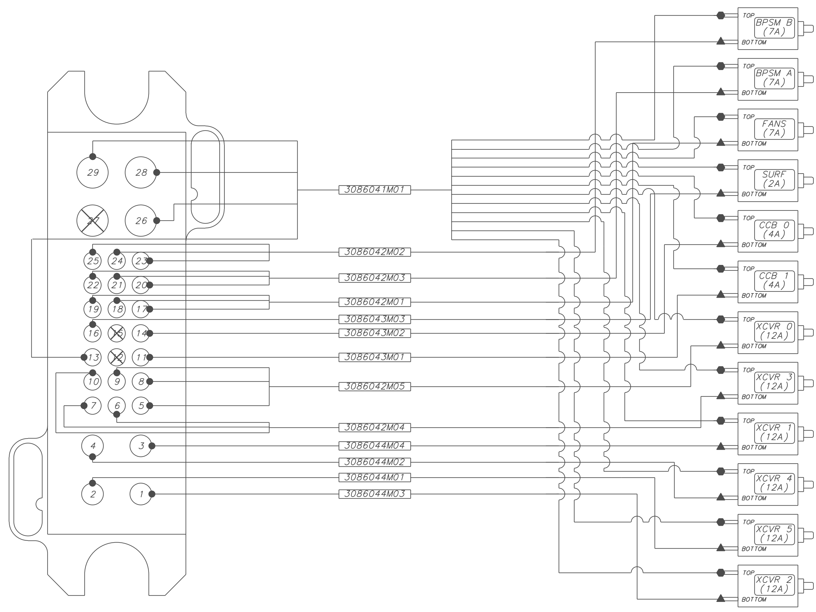
CIRCUIT BREAKER/CABLE HARNESS WIRING SCHEDULE
