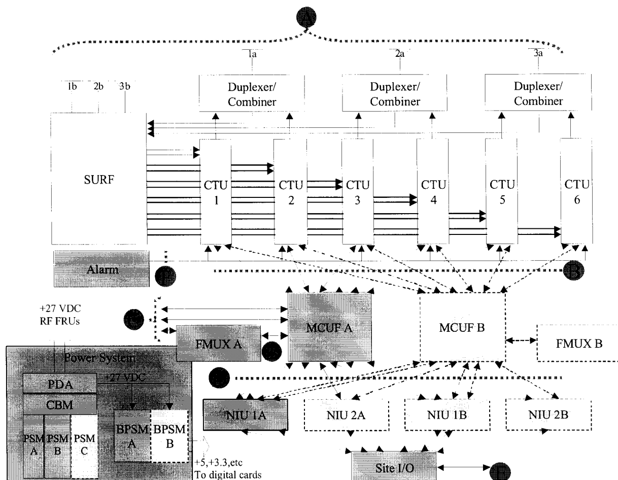
Figure 1 HorizonMacro Hardware Block Diagram
