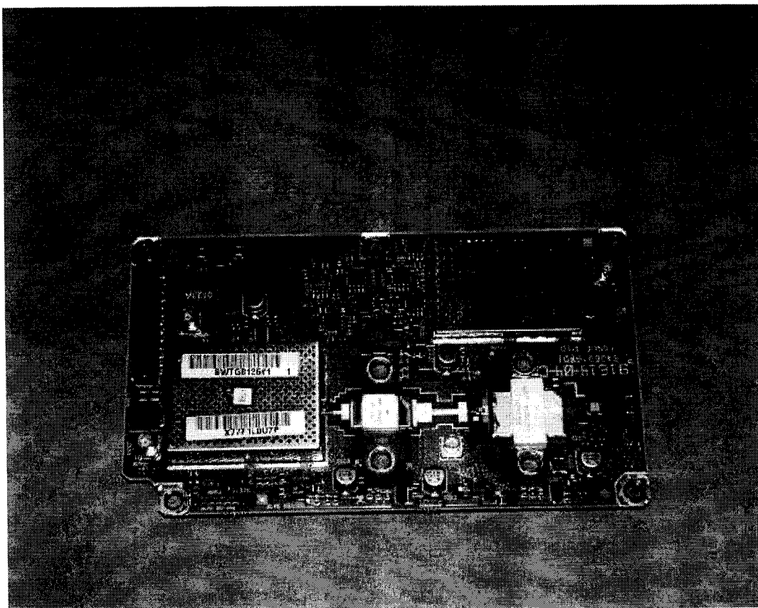
IHET6BV1 HorizonMacro1900 Transceiver Power Supply Board View
