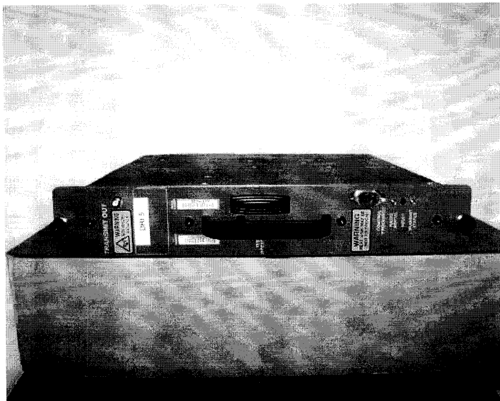
IHET6BV1 HorizonMacro1900 Transceiver Front View
