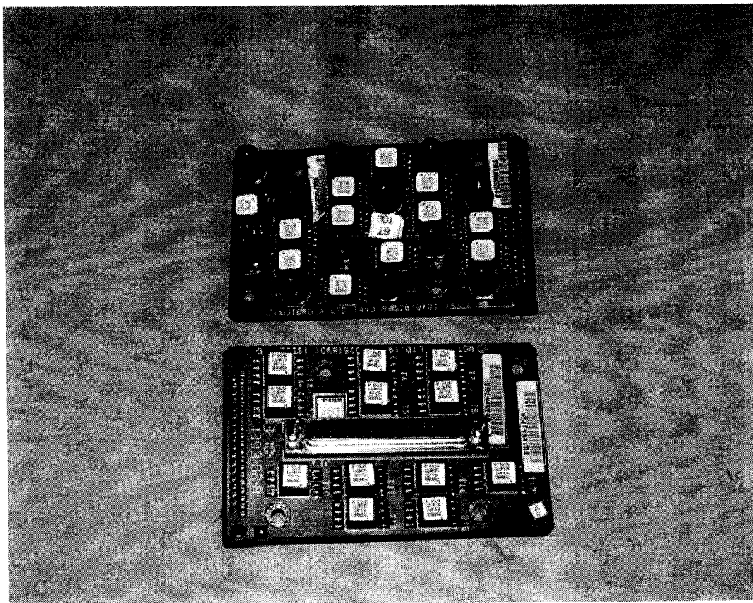
IHET6BV1 HorizonMacro1900 Line Interface Cards Front View
