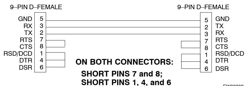
Figure 1-5: Null Modem Cable Detail
