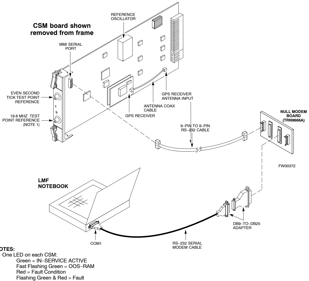
Figure 3-12: CSM MMI terminal connection
