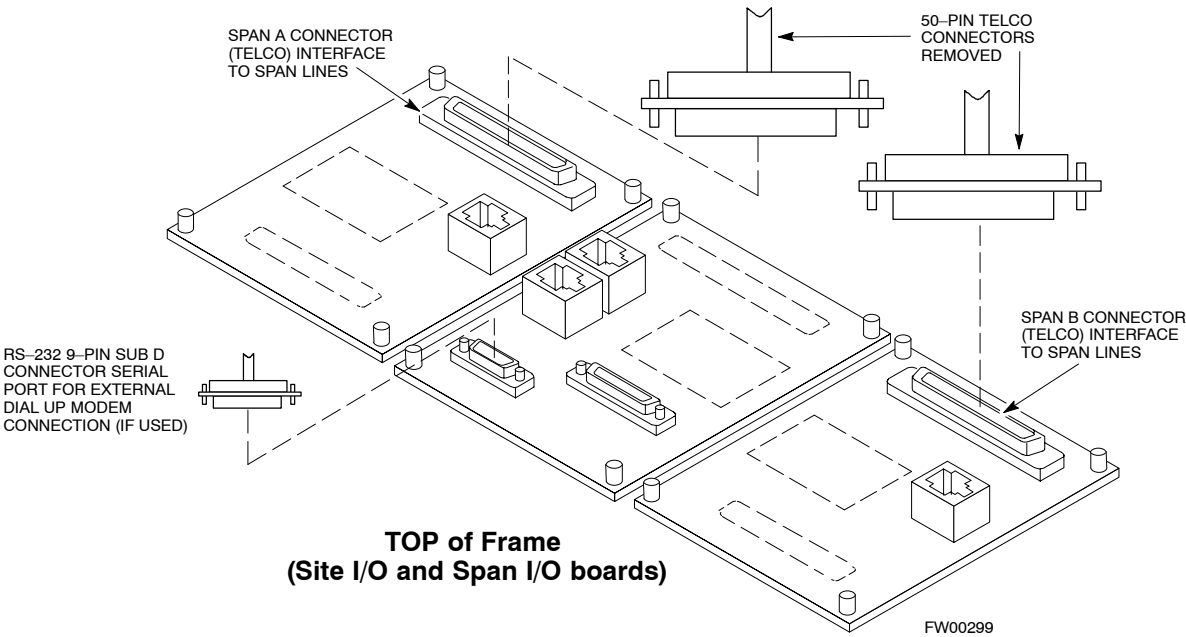
Figure 3-2: Span I/O Board Span Isolation
