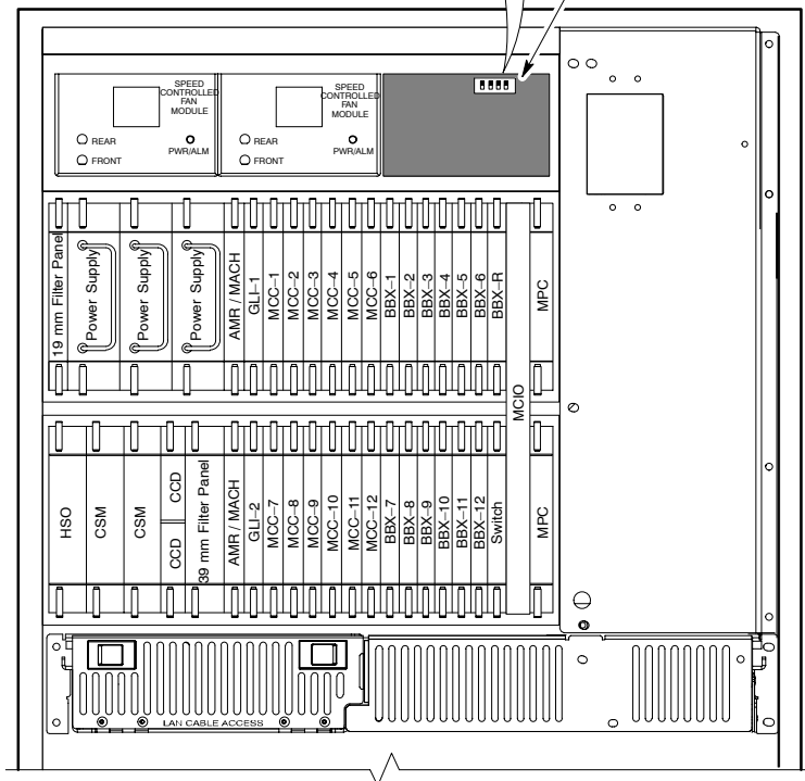
SC 4812T C-CCP SHELF
