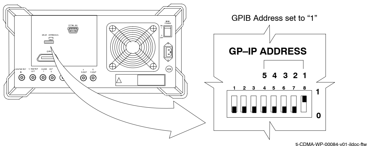
Figure F-6: Advantest R3562 GPIB Address Switch Setting
