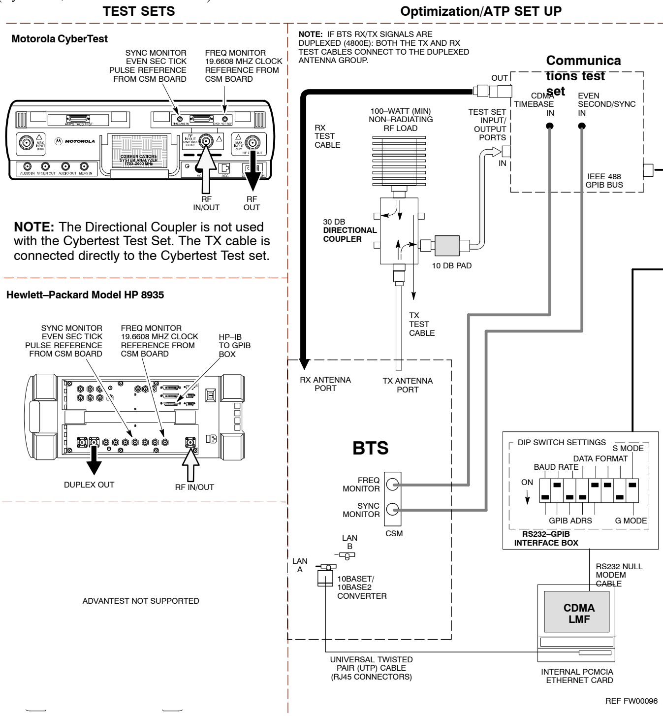
Figure 3-18: IS-95 A/B Optimization/ATP Test Setup Calibration Using Directional Coupler (CyberTest, HP 8935 and Advantest)
