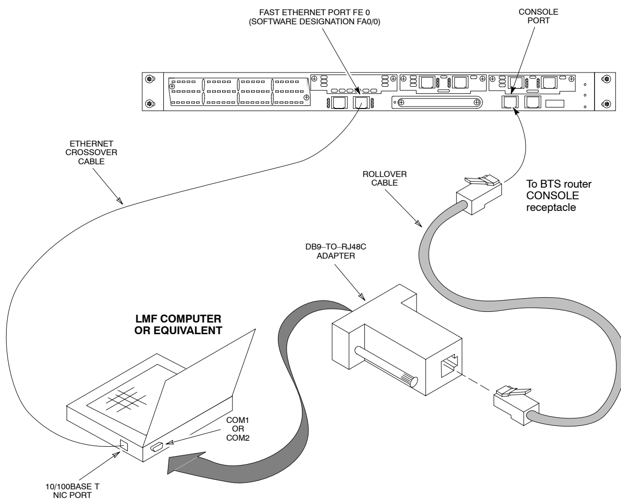
Figure I-4: LMF Computer TFTP Connections to BTS Router
