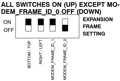
Figure 2-2: Backplane DIP Switch Settings
