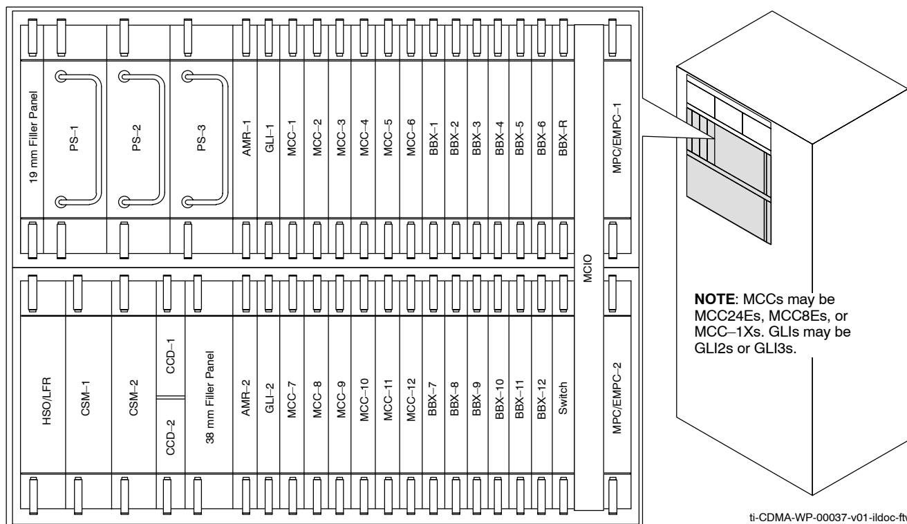
Figure 3-26: C-CCP Shelf
