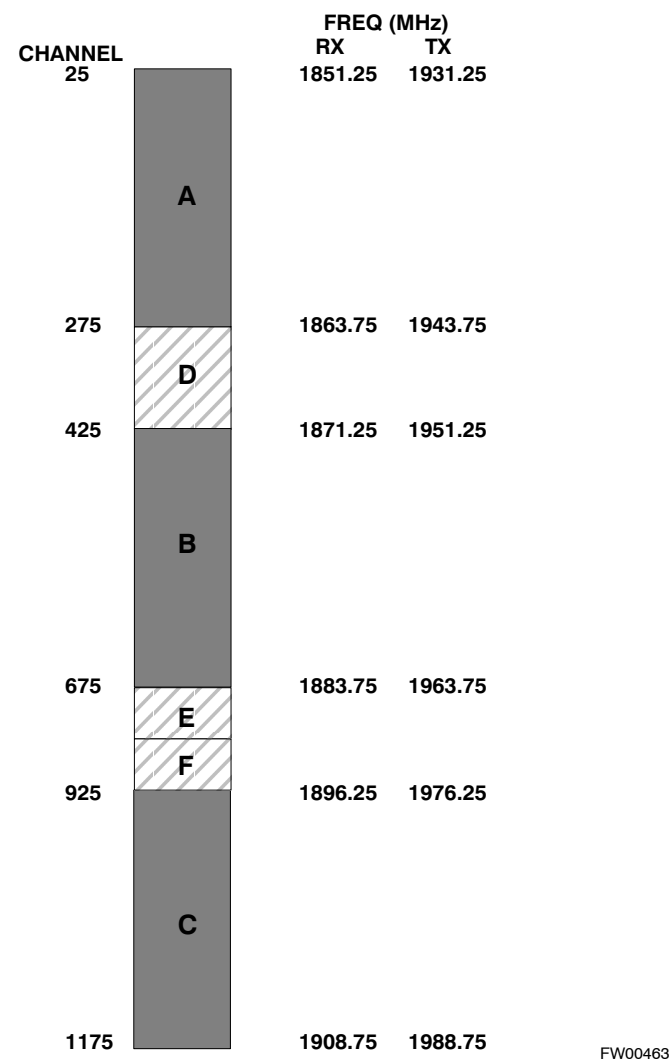
Figure E-1: North America PCS Frequency Spectrum (CDMA Allocation)
