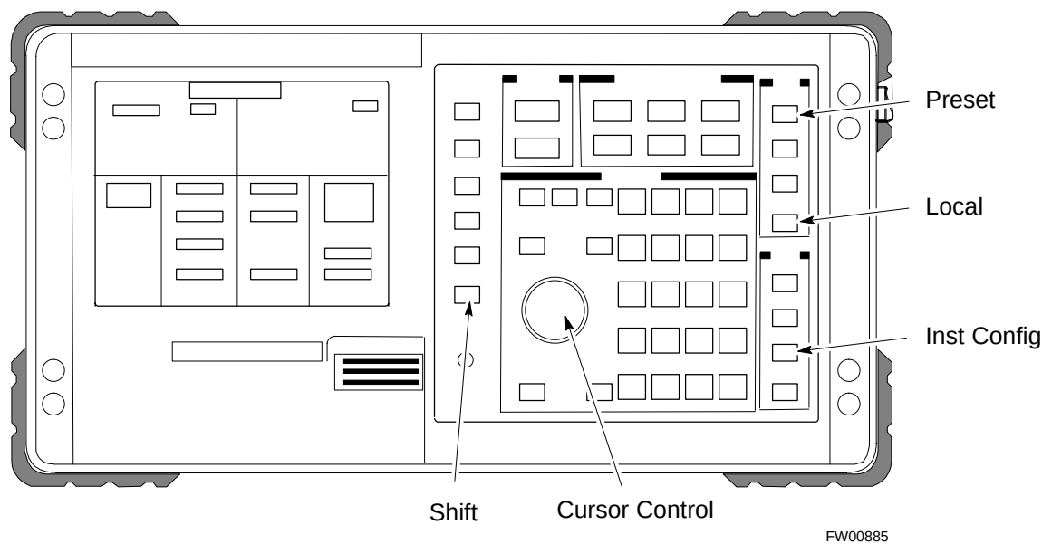
Figure I-3: HP8935 Test Set
