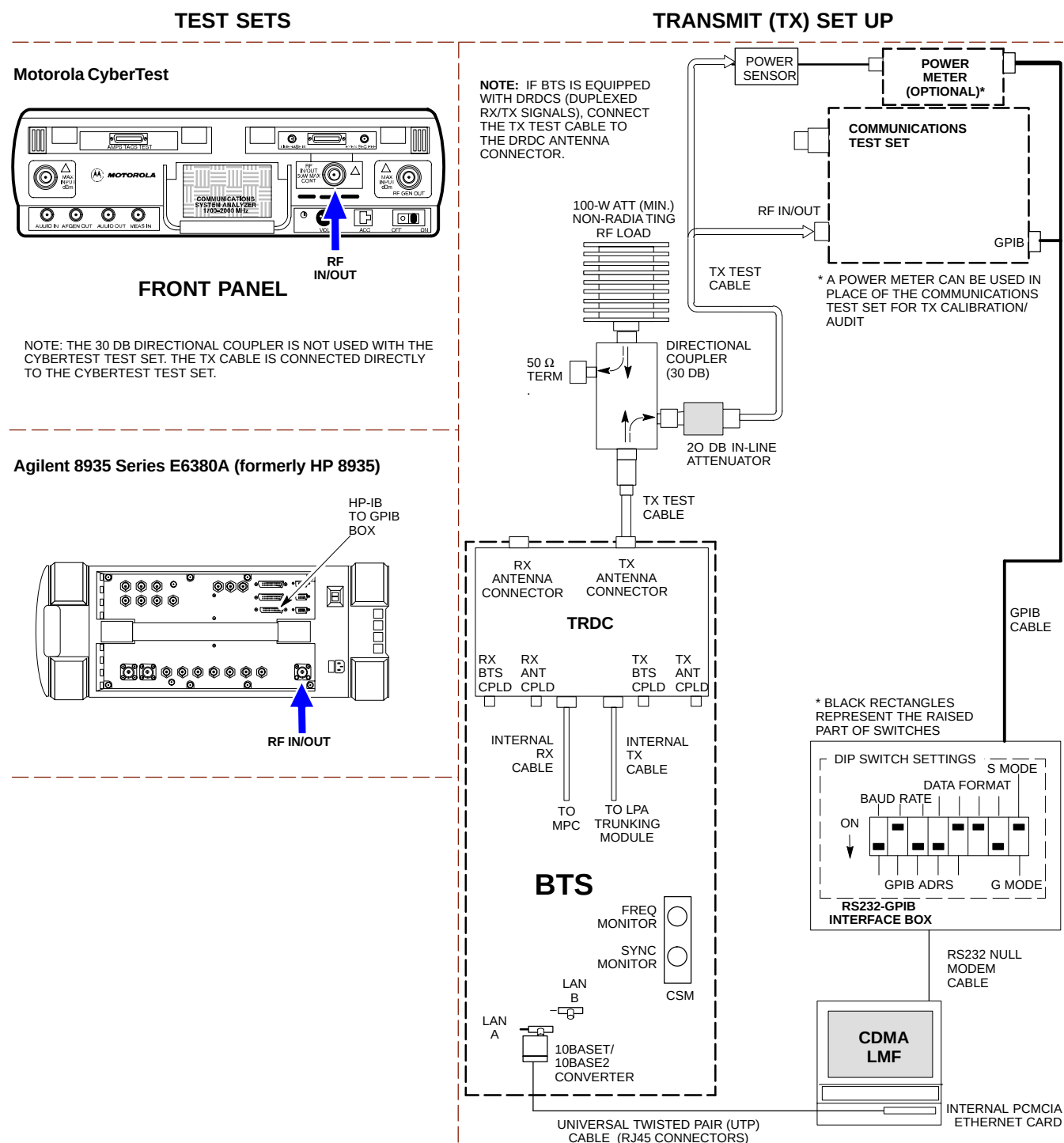
Figure 3-10: TX Calibration Test Setup - CyberTest (IS-95A/B) and Agilent 8935 (IS-95A/B and CDMA2000 1X)
