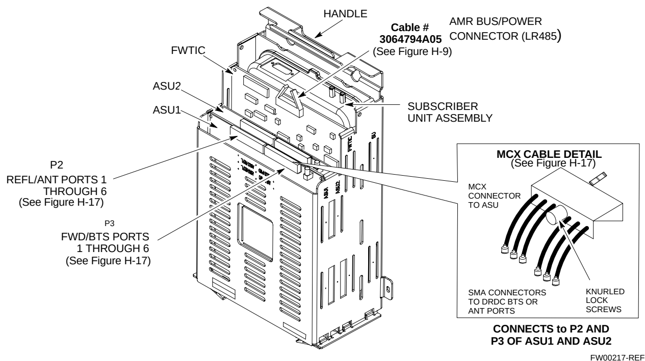
Figure H-16: RFDS Component Identification
