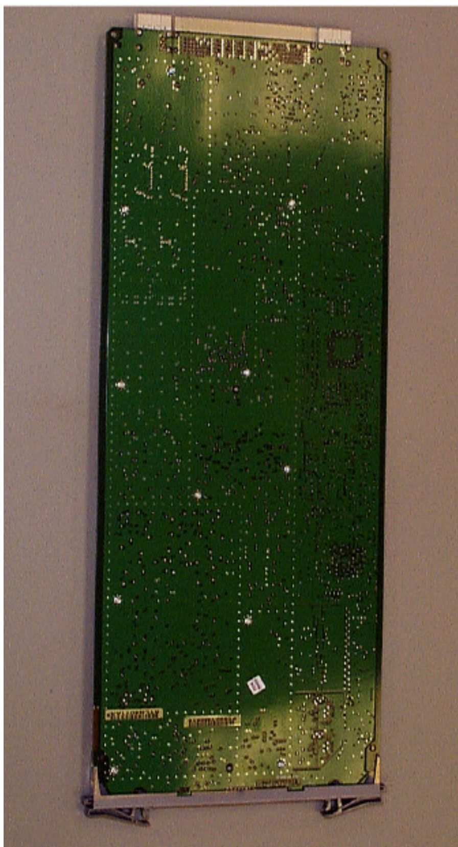
IHET6YR1 SC4812T 1.9 GHz BBX2 Back
