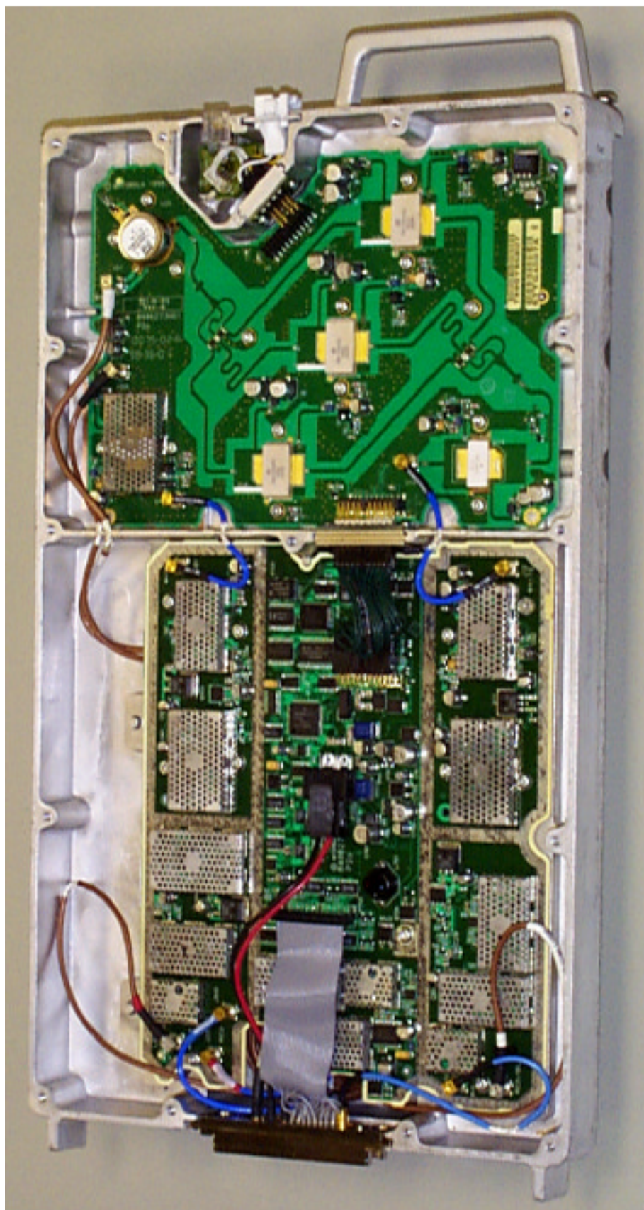
IHET6YR1 SC4812T 1.9 GHz LPA without Cover
