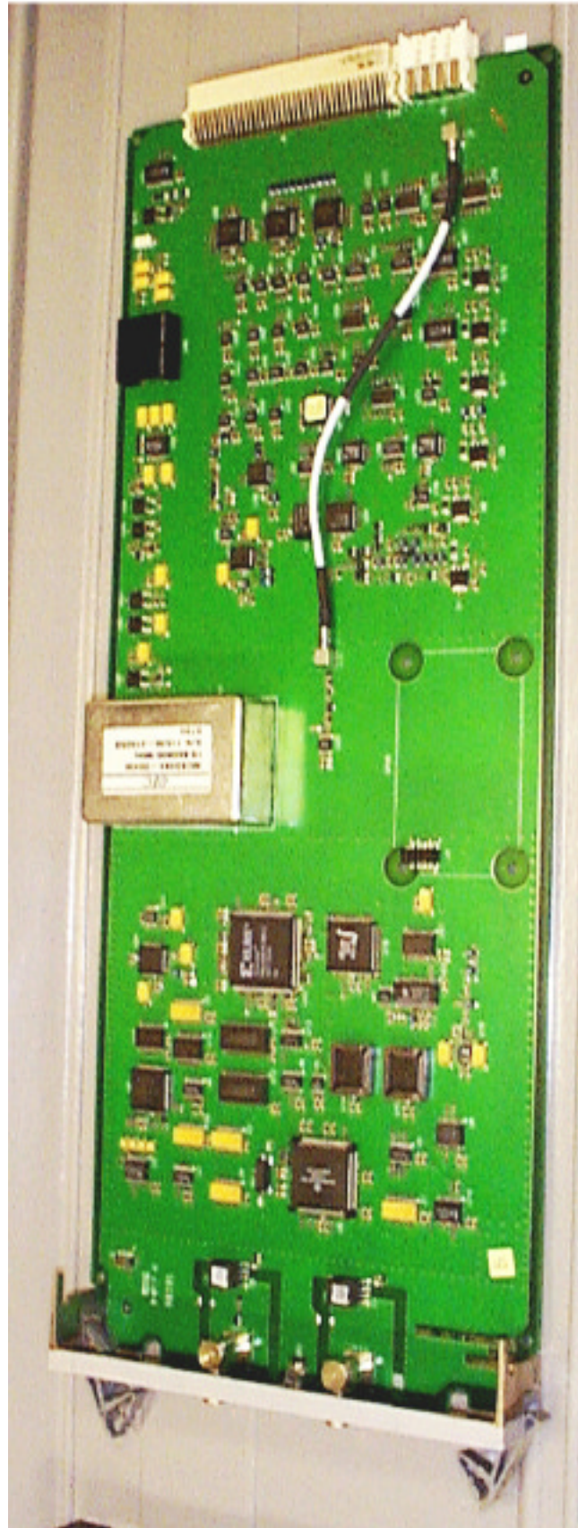
IHET6YR1 SC4812T 1.9 GHz CSM2 Front
