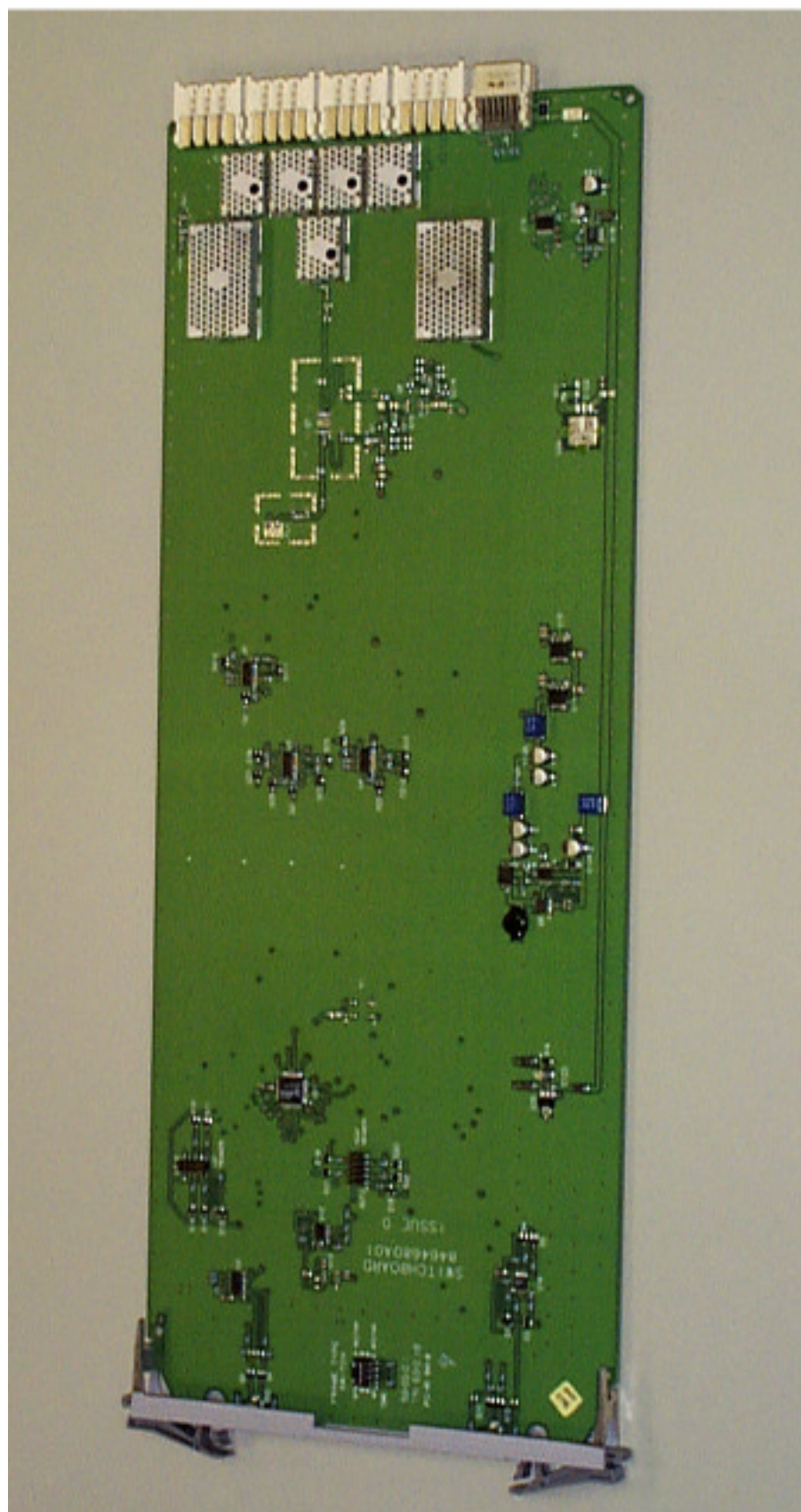
IHET6YR1 SC4812T 1.9 GHz Switch Card Front
