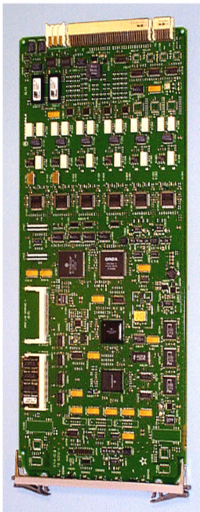
IHET6YR1 SC4812T 1.9 GHz GLI2 Front
