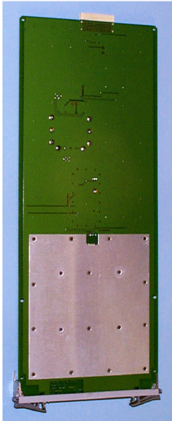
IHET6YR1 SC4812T 1.9 GHz HSO Back
