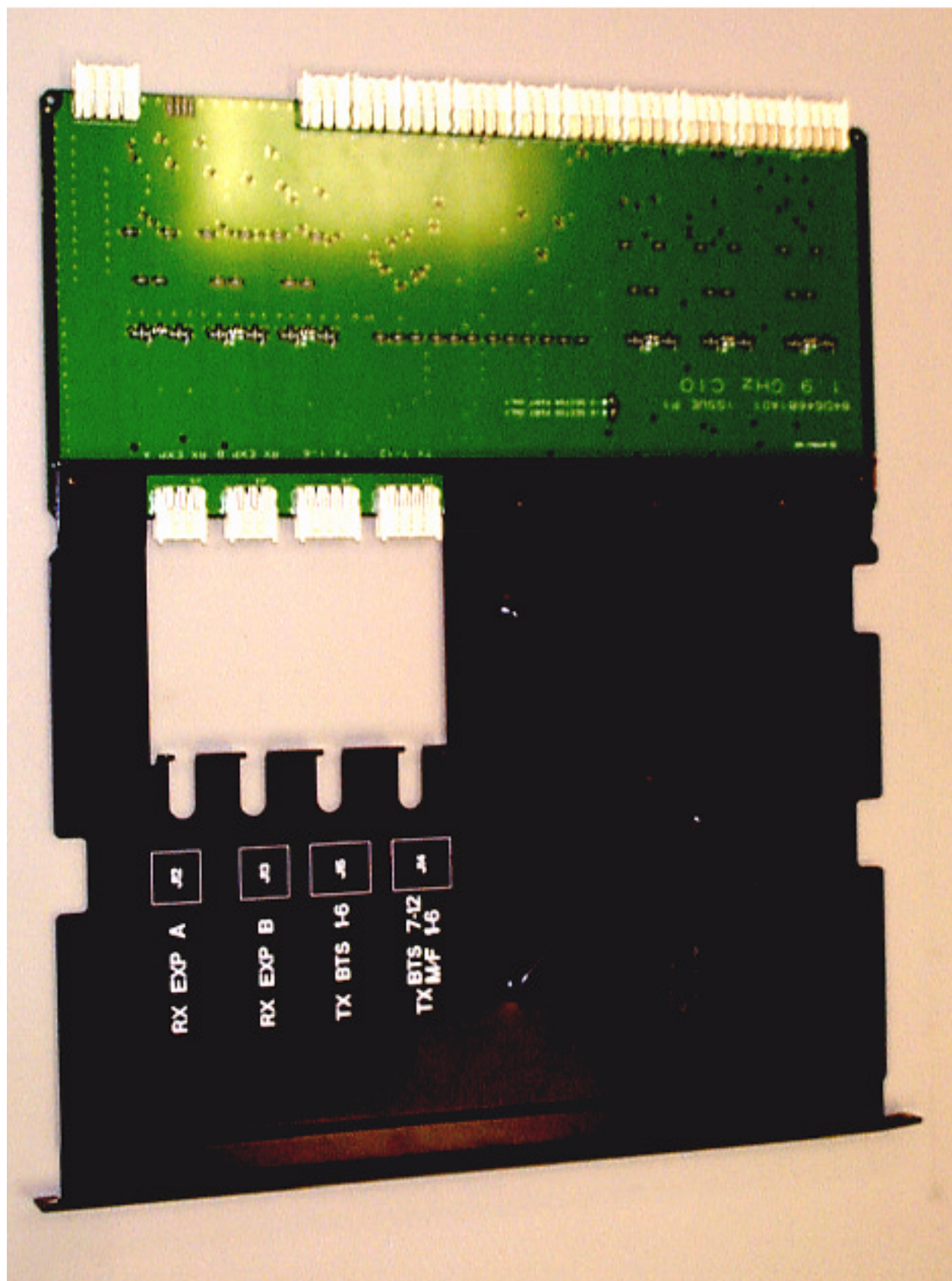
IHET6YR1 SC4812T 1.9 GHz CIO Front
