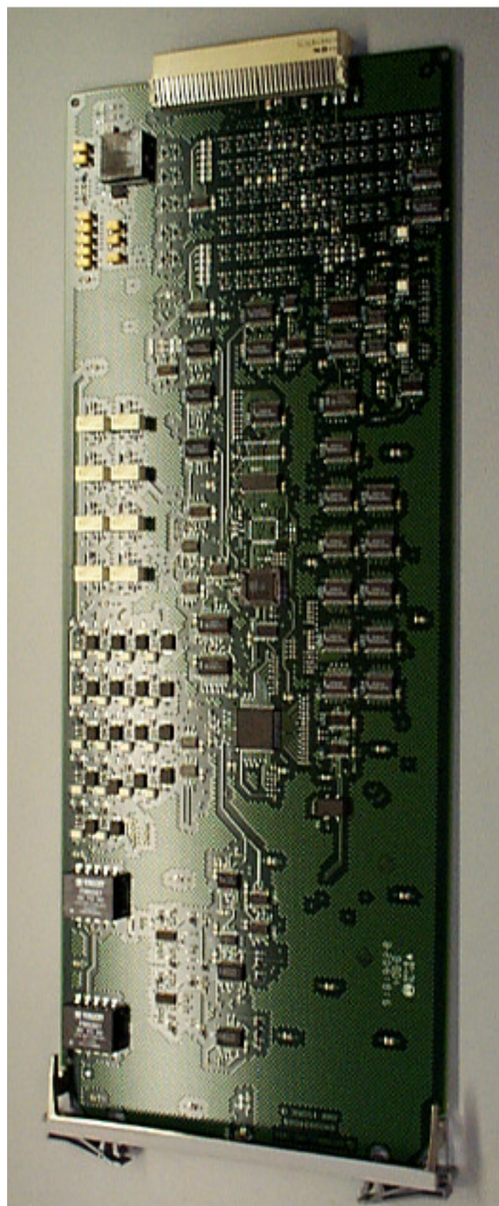
IHET6YR1 SC4812T 1.9 GHz AMR Front
