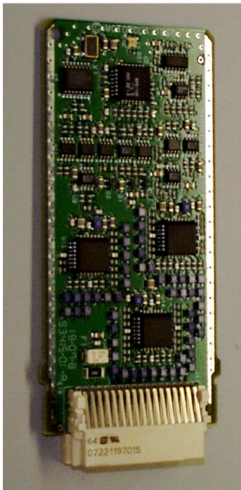
IHET6YR1 SC4812T 1.9 GHz CCD Front
