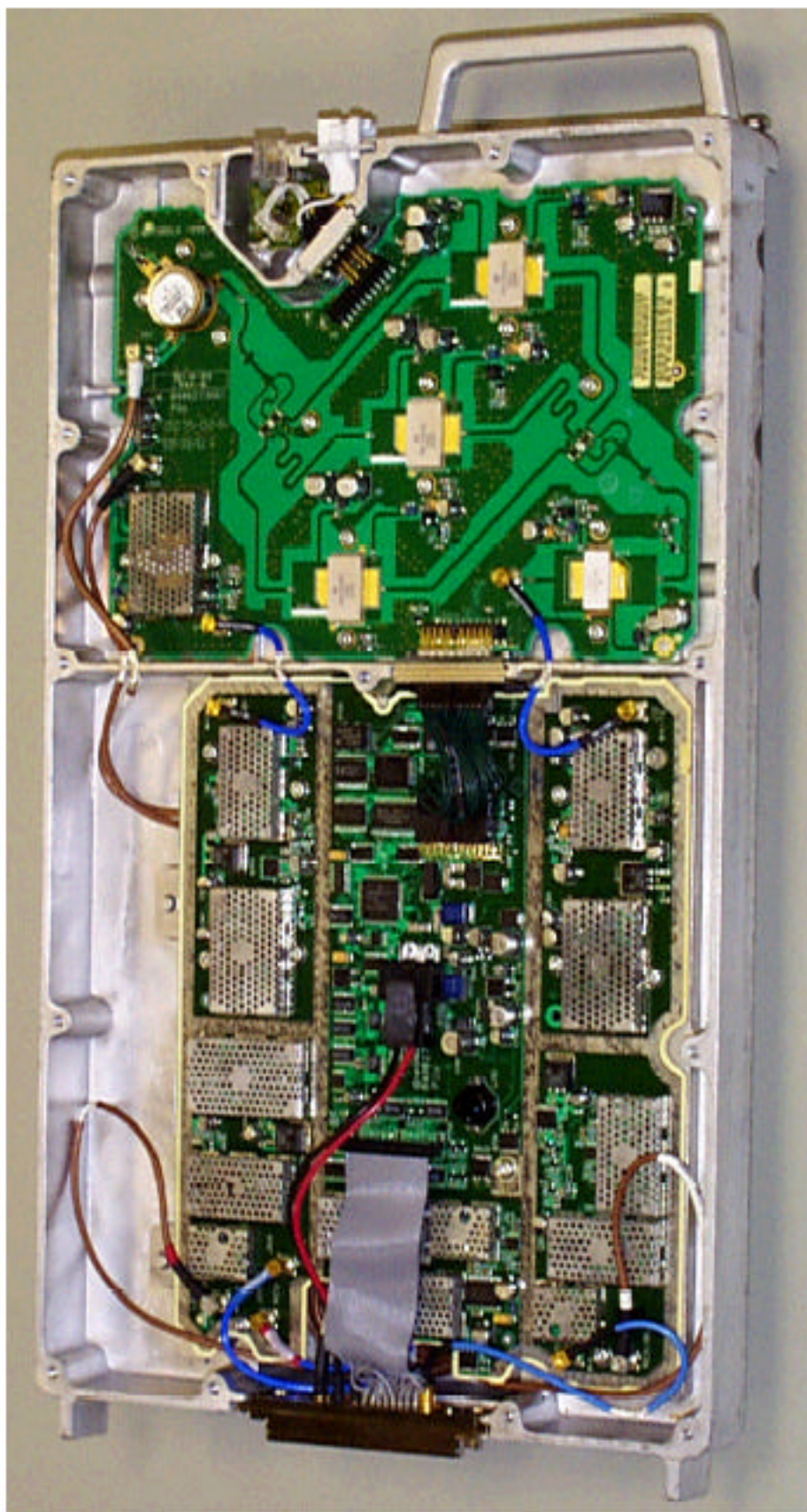
IHET6YZ1 SC4812ET 1.9 GHz LPA without Cover
