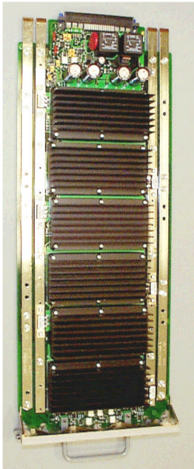
IHET6YZ1 SC4812ET 1.9 GHz Power Supply Front
