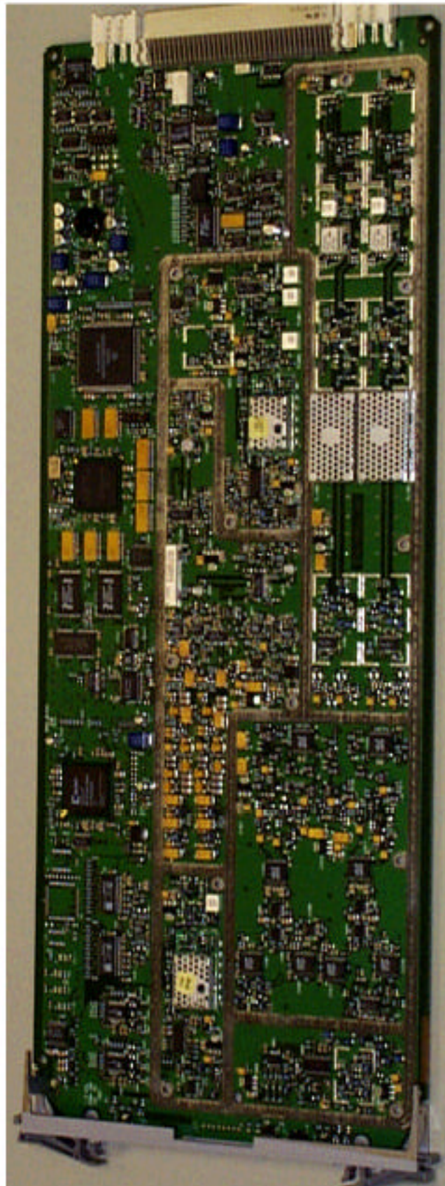
IHET6YZ1 SC4812ET 1.9 GHz BBX2 without Cover
