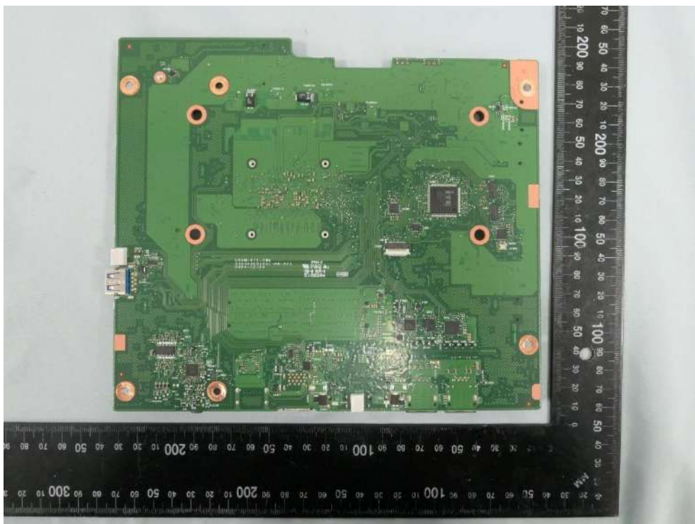
(28) EUT Photo
