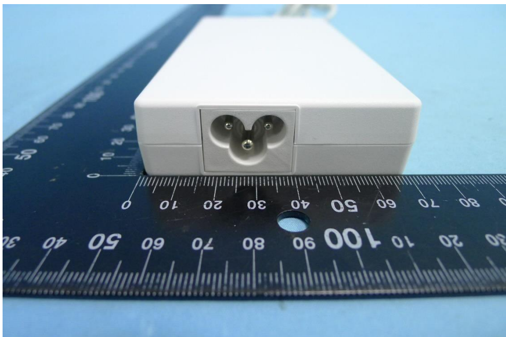
(10) EUT Photo(Adapter)
