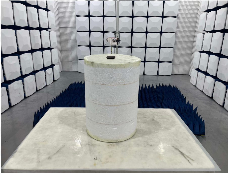
Setup3 Above 18 GHz
