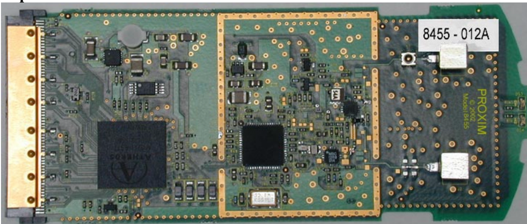
Top Side PCB without Shield:
