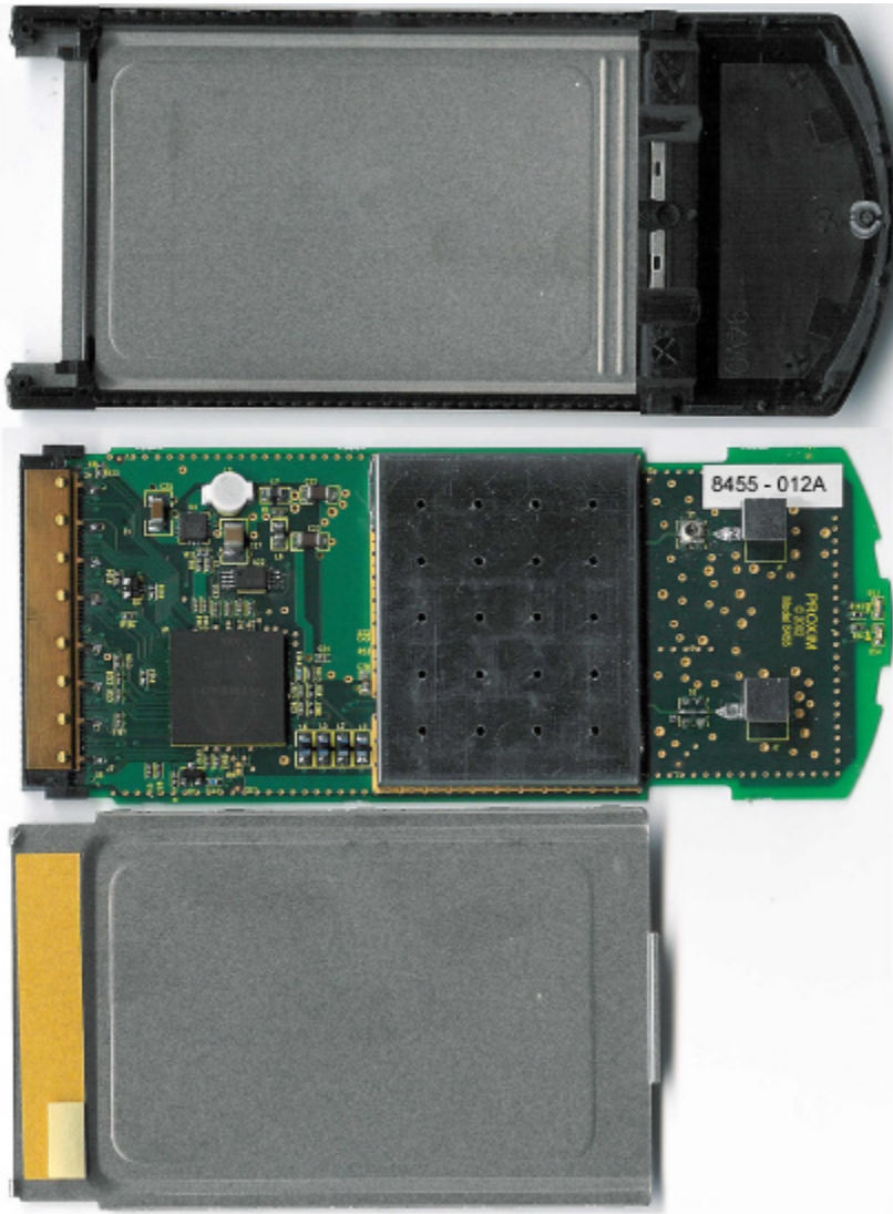
Inside View of Covers and PCB:
