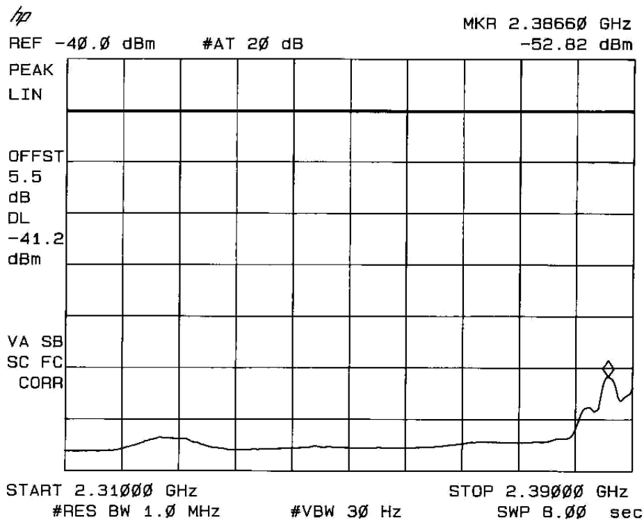
Figure 9.1: average values in restricted band, All bitrate settings, conducted measurement, corrected for 2 dBi antenna gain and 2.6 dB cable losses. 54 dBμV/m :: -41.2 dBm display line setting.
