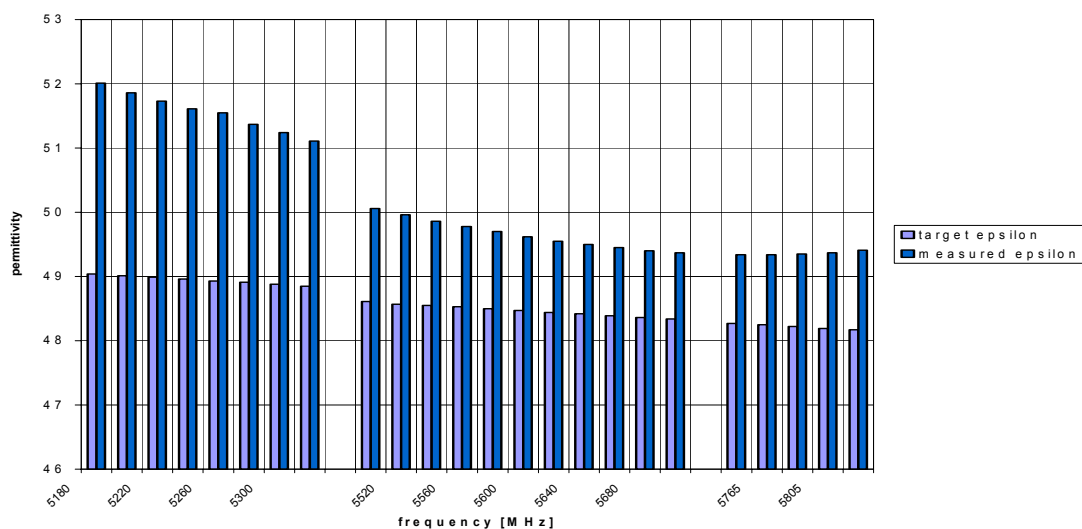
5 GHz body liquid validation
