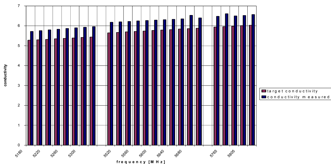
5 GHz body liquid validation
