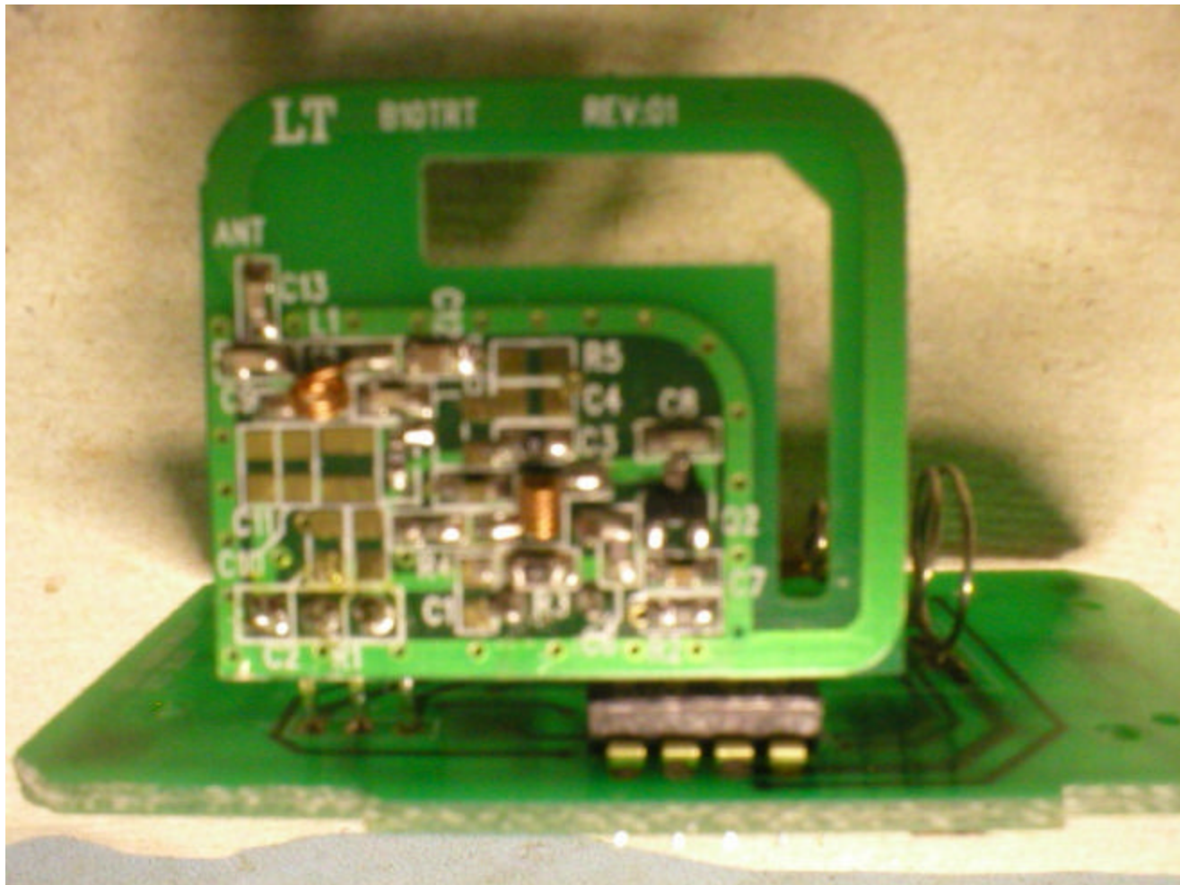
Internal Photo - Transmitter Board Component Side Model 85773 (B21W) FCC ID: IN2TX20
