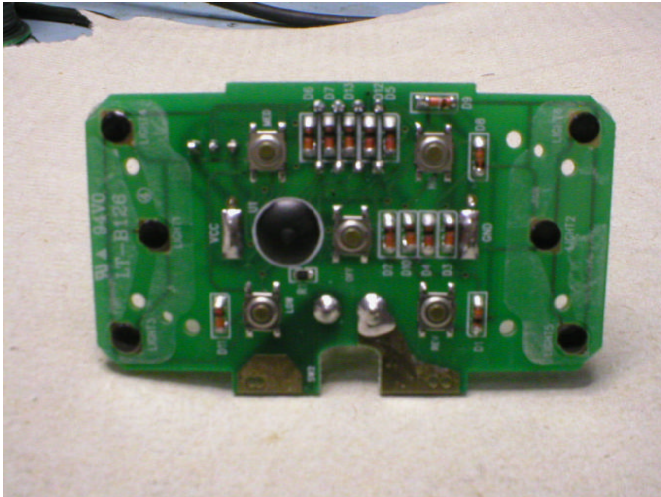
Internal Photo - Main Board Component Side Model 85773 (B21W) FCC ID: IN2TX20
