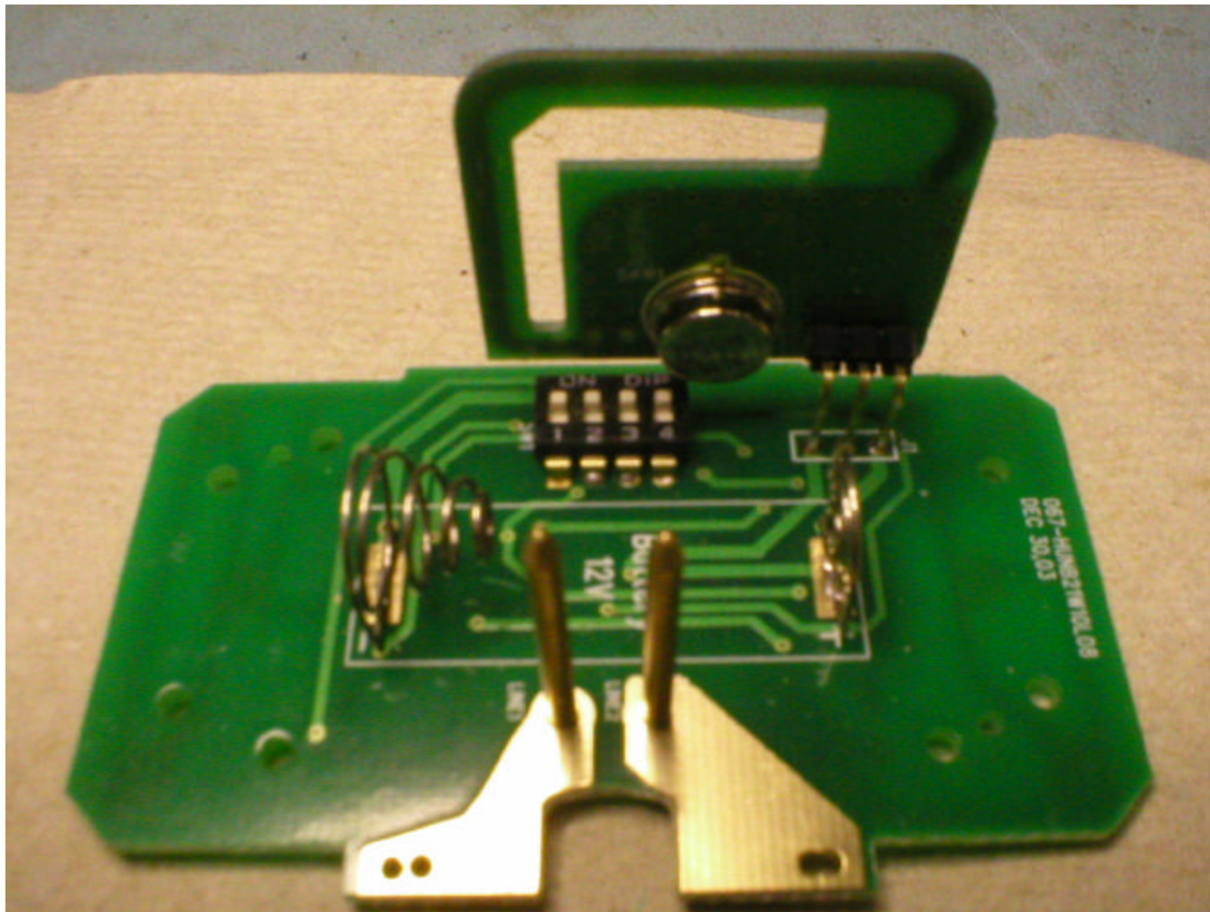
Internal Photo - Main Board Solder Side Model 85773 (B21W) FCC ID: IN2TX20
