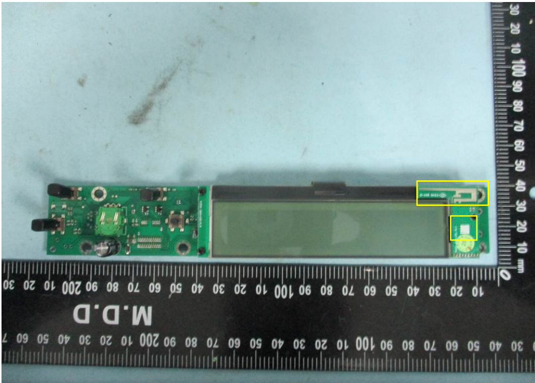
(19) 2.4G ANT and RF chip
