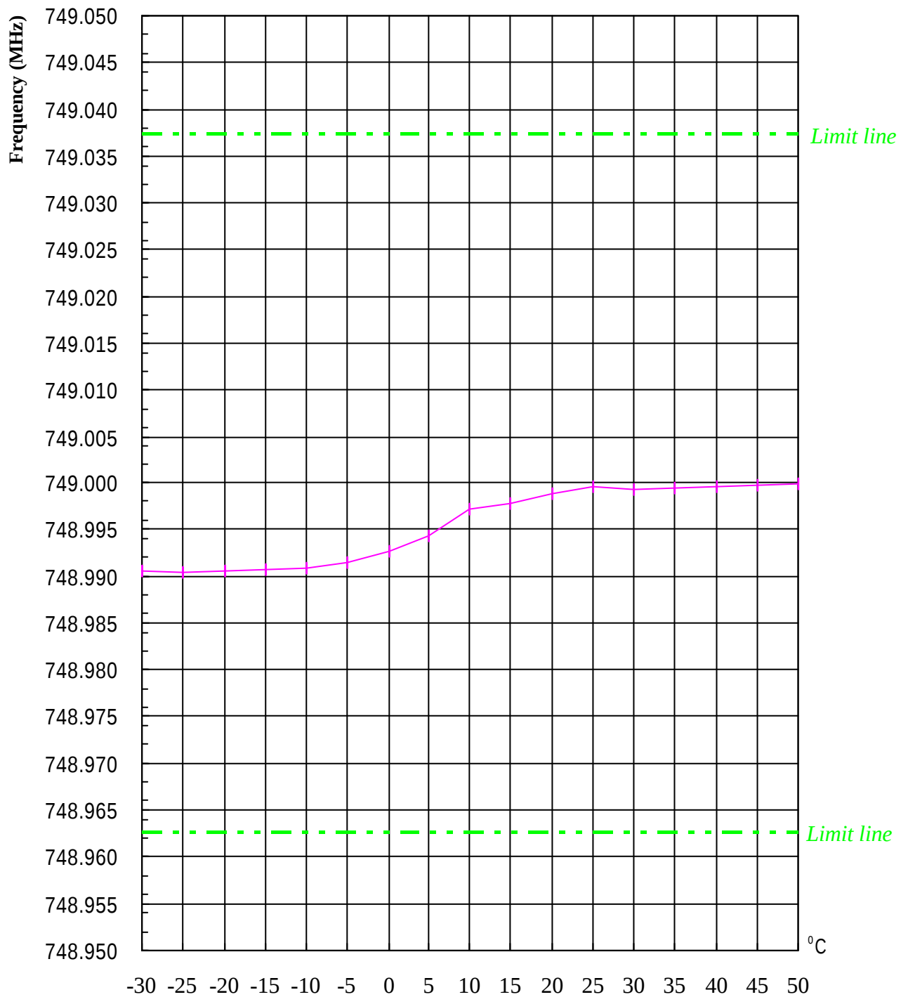
Chart 7.1 Temperatuer Variation Vs. Frequency
