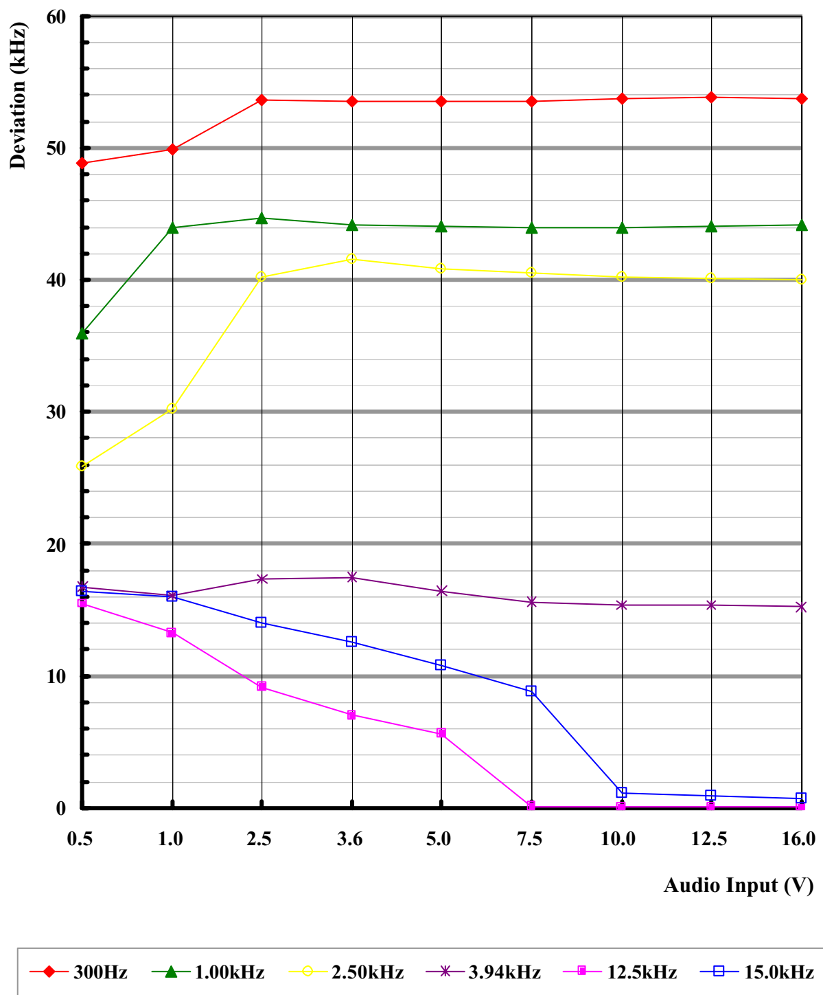
Chart 4.2 Modulation Limiting Measurement Positive
