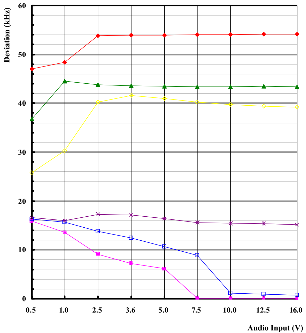
Chart 4.1 Modulation Limiting Measurement Negative
