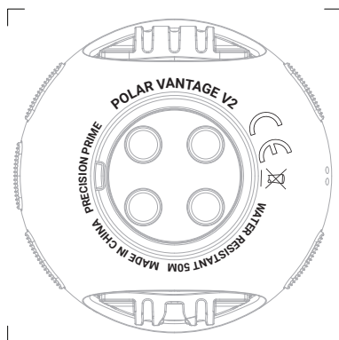
Laser markings position
