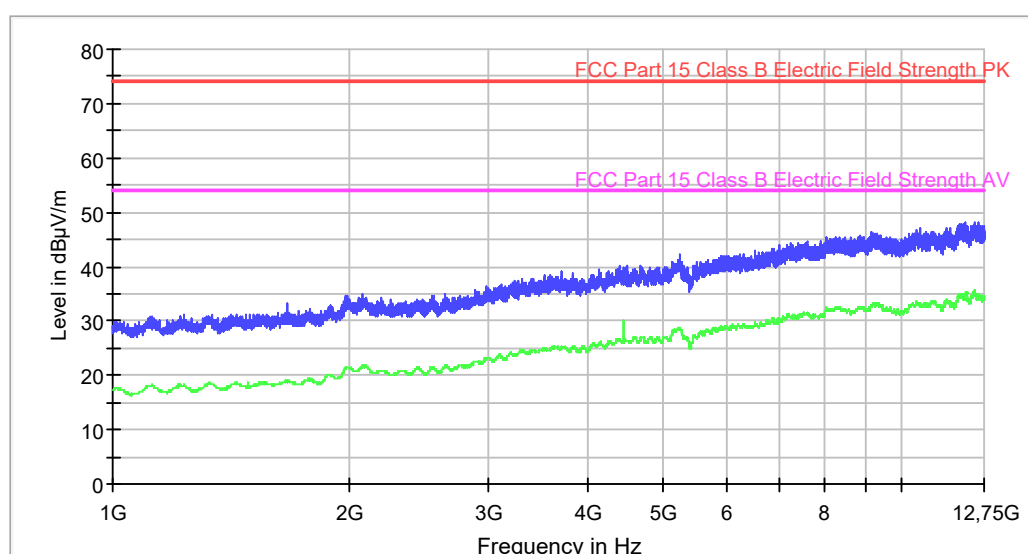
RE FCC Part 15 ClassB 1-12,75 GHz
