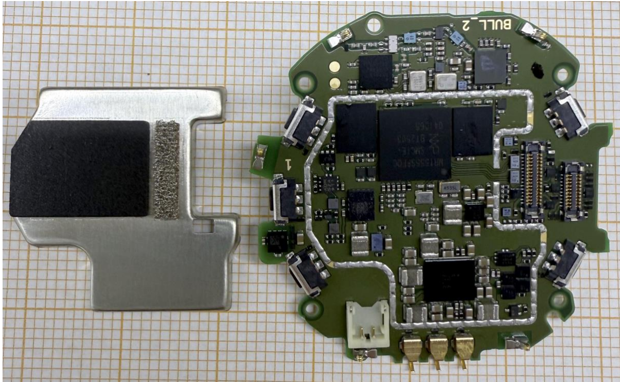
Figure 8. The main PWB from component side with RF shield removed.
