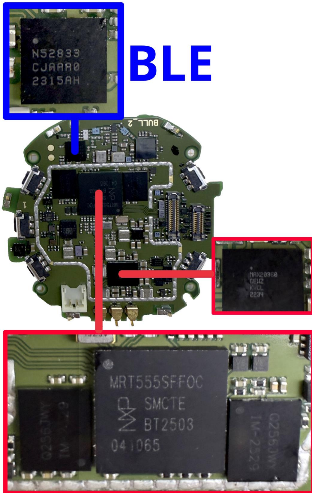
Figure 10. Main PWB component details.
