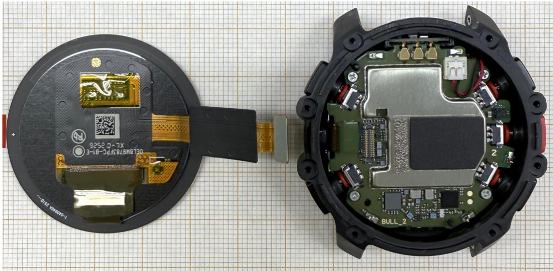
Figure 3. Display module separated.
