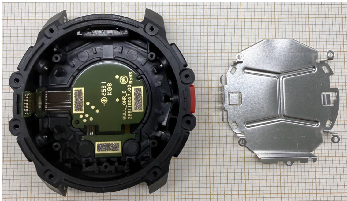
Figure 12. Battery shield removed, OHR PWB visible.
