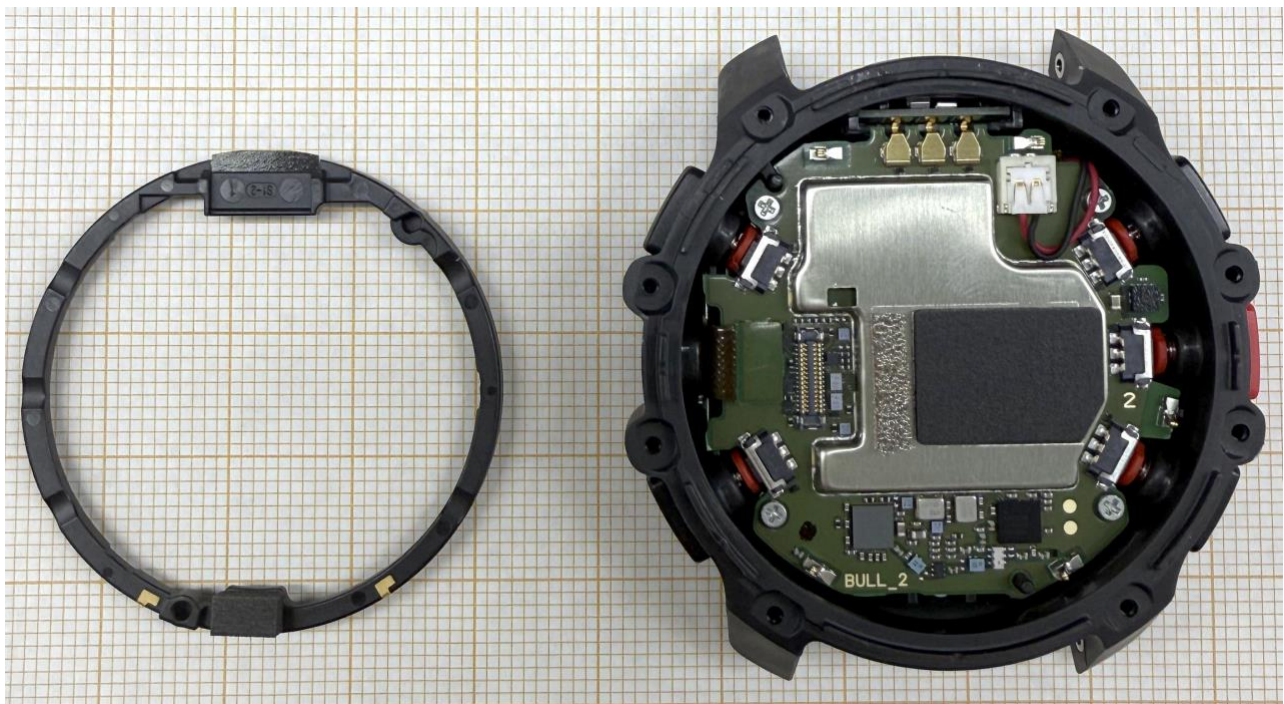
Figure 4. Antenna frame separated.
