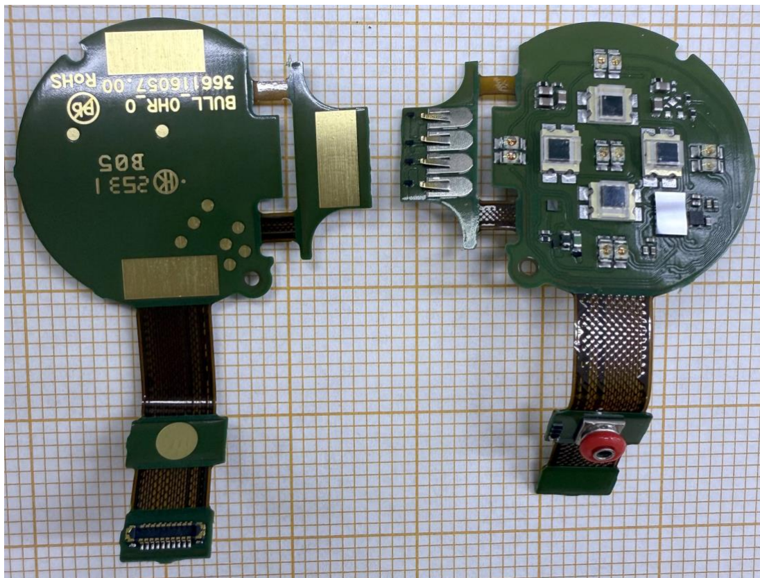
Figure 14. Both sides of the OHR PWB.
