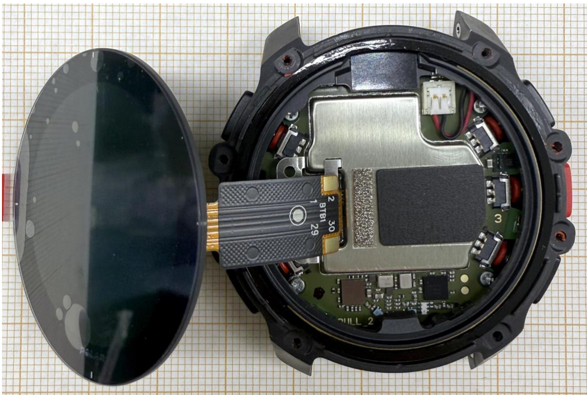
Figure 2. Device opened, display cable attached.
