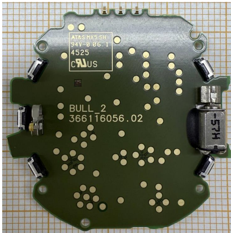
Figure 9. The main PWB from bottom side.
