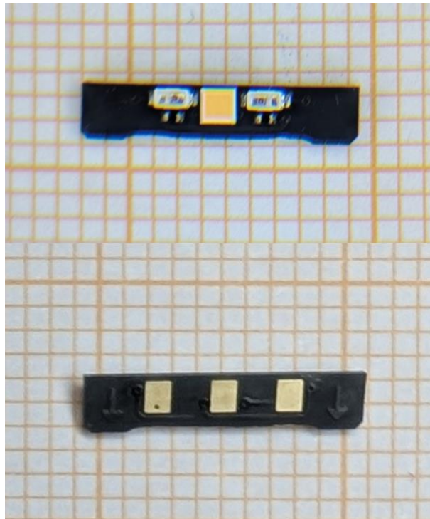
Figure 15. Flashlight PWB from both sides.
