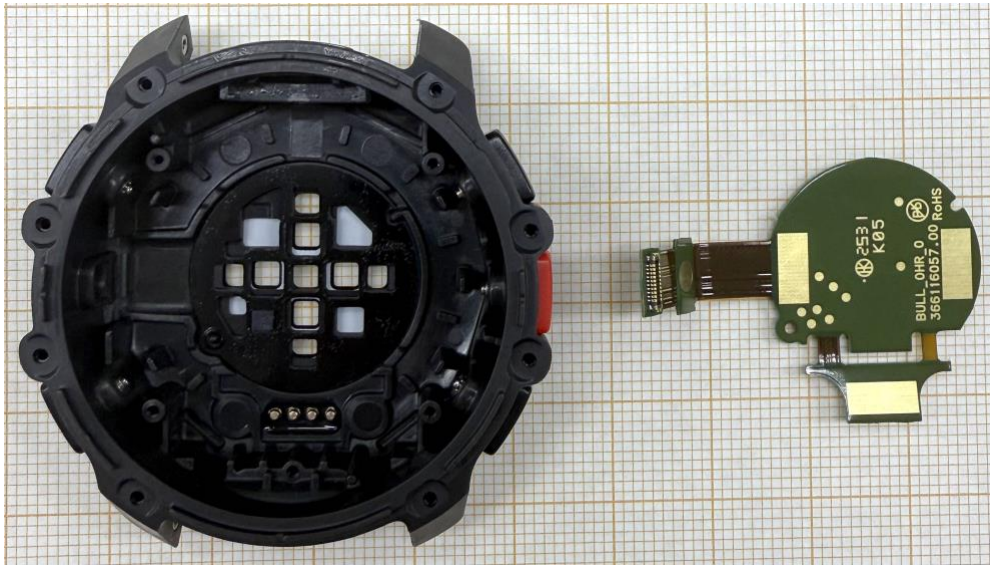
Figure 13. OHR PWB removed from the case.
