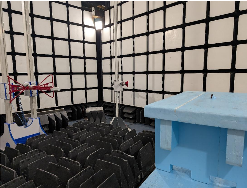
Figure 4. Test setup for (RSE) radiated emissions in full-anechoic chamber, 1 GHz - 25 GHz.
