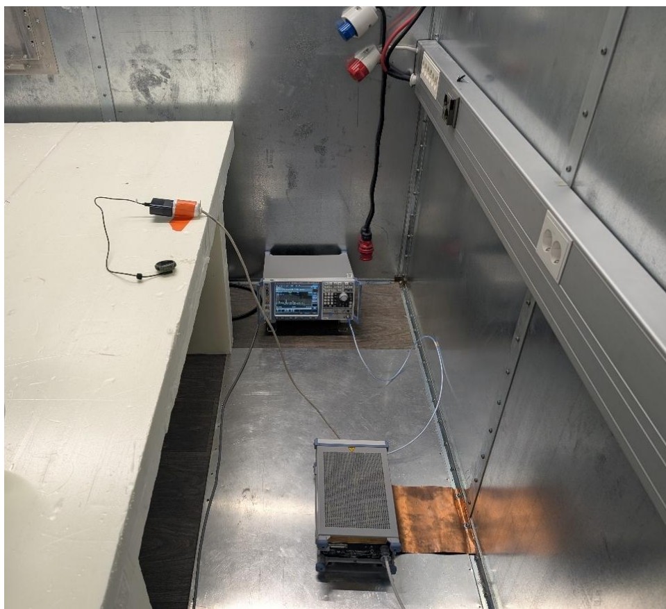
Figure 5. Test setup for AC conducted emissions.
