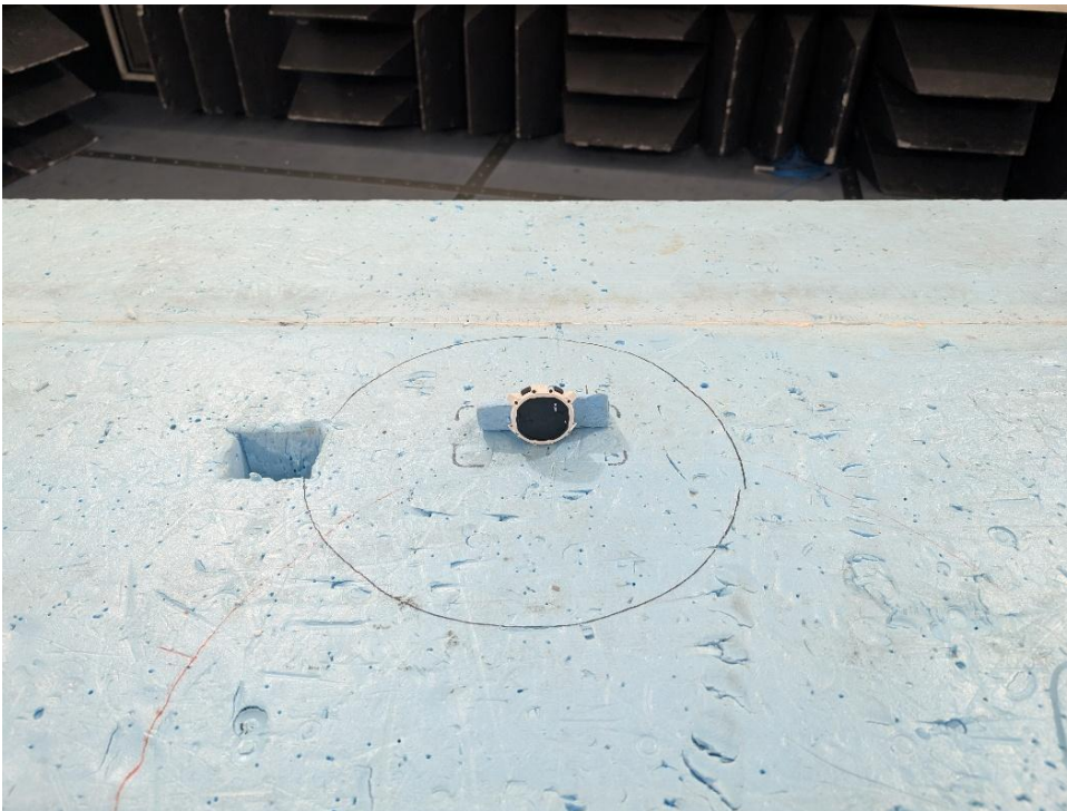
Figure 8. EUT in Z orthogonal position.
