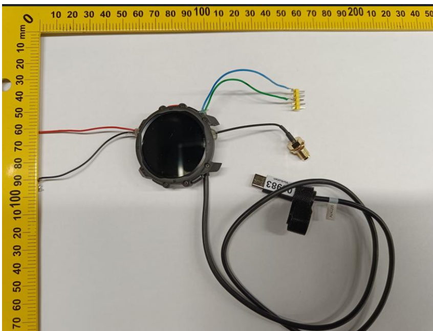
Figure 2. Conducted RF EUT.
