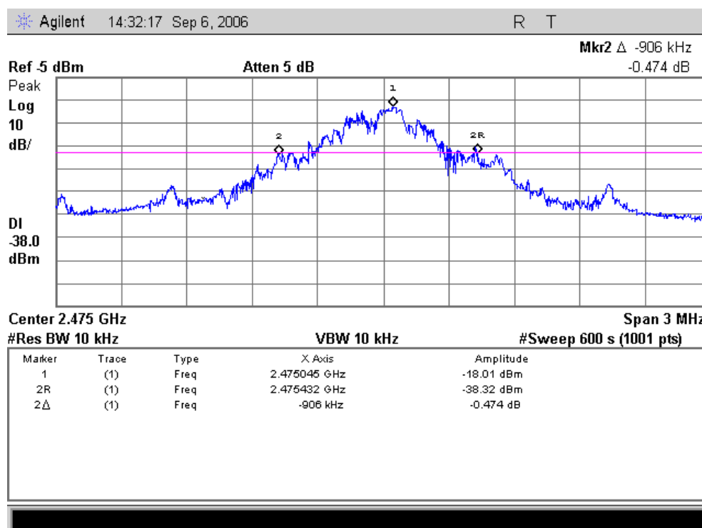
Picture 3: 20dB Bandwidth measurement result
