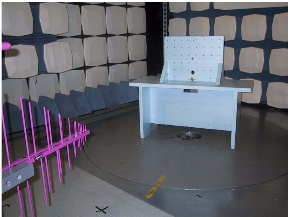
Picture 2: Spurious emission and field strength measurement setup
