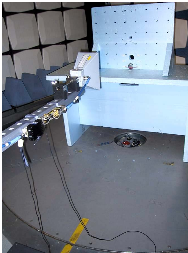
Picture 1: Spurious emission measurement setup
