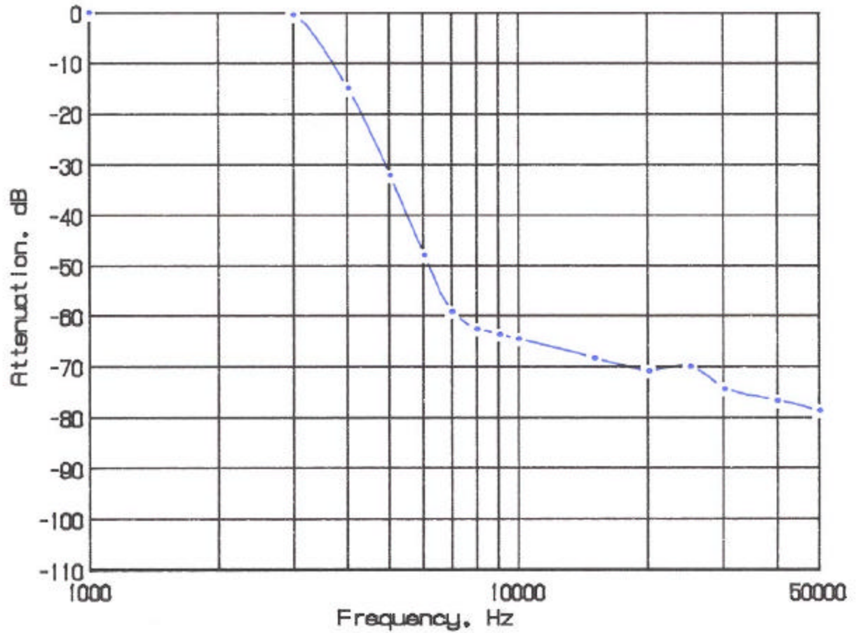
FIGURE 3 AUDIO LOW PASS FILTER RESPONSE
