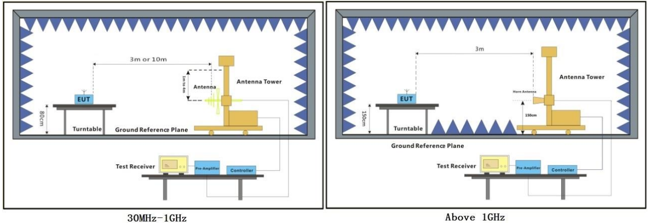
30MHz-1GHz
