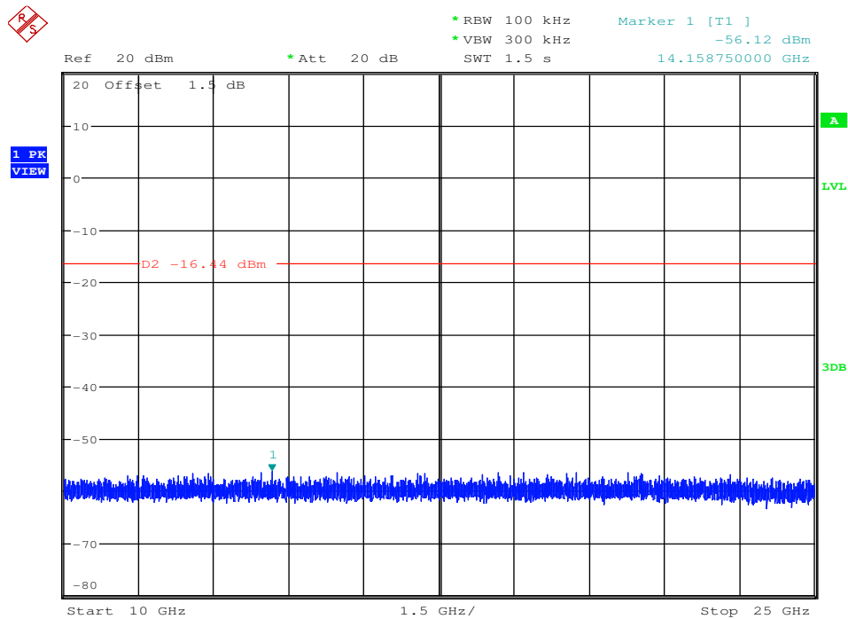
RF Conducted Spurious Emissions_11B_2437_Ant1
