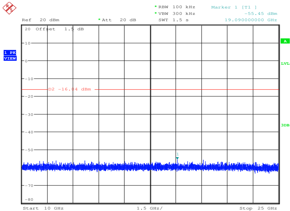
RF Conducted Spurious Emissions_11G_2412_Ant1
