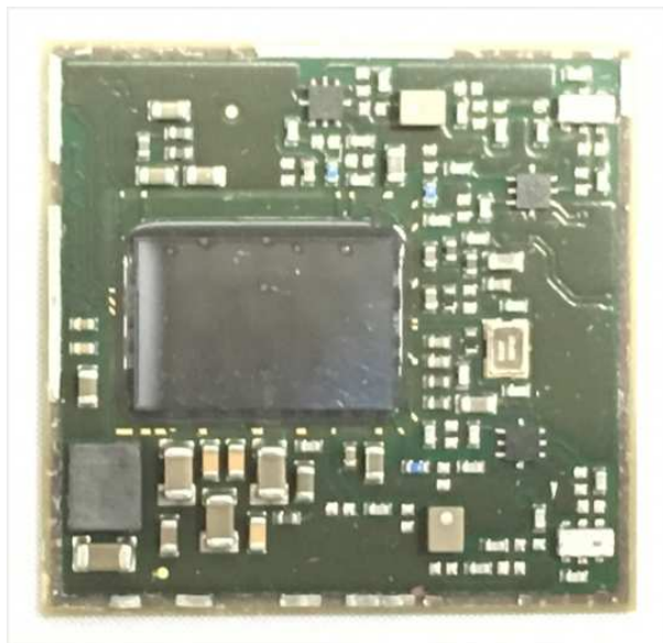
Radio Module (without shielding case)
