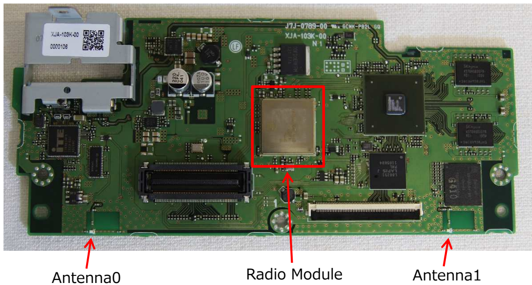
PCB(A-side) with Radio module for DMX958XR
