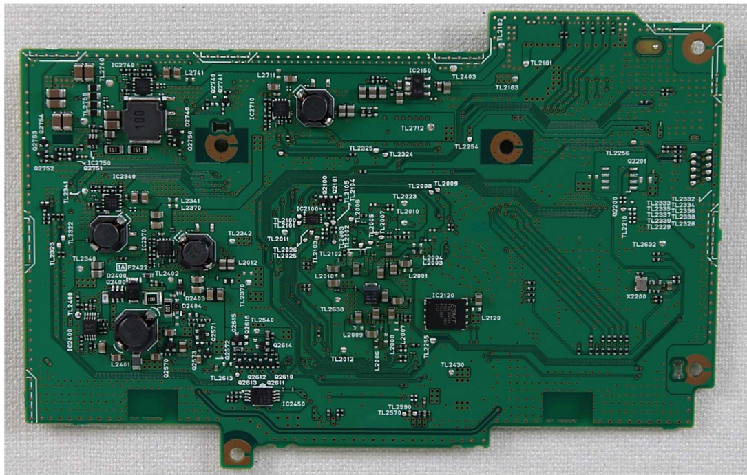
PCB(B-side) with Radio module
