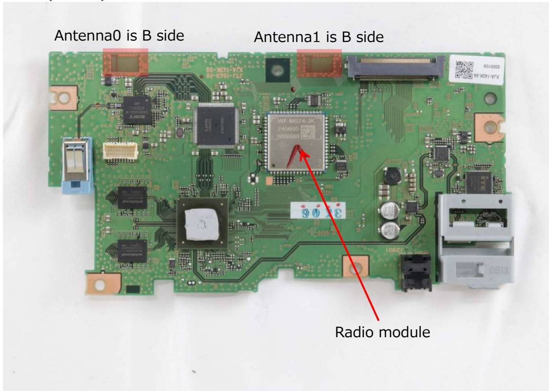
PCB(A-side) with Radio module
