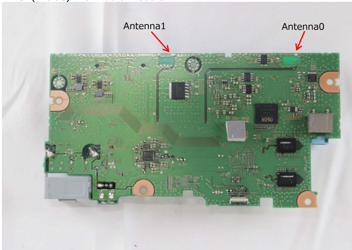
PCB(B-side) with Radio module
