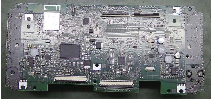
Panel Unit 1 (Side A)
