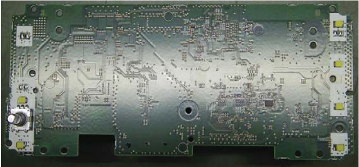
Panel Unit 2 (Side B)
