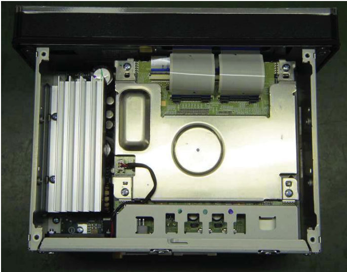
Top cover disassembly
