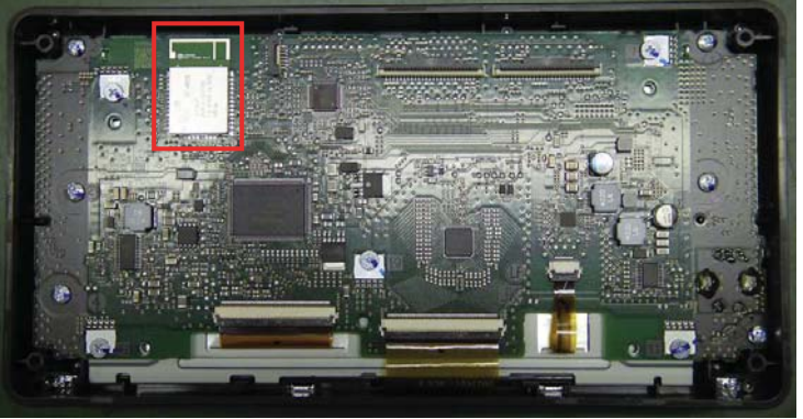
Panel assembly 2 (without case)
