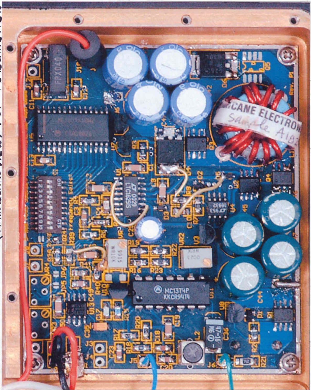
PHOTOGRAPH 4: TOP VIEW OF MAIN PC BOARD
