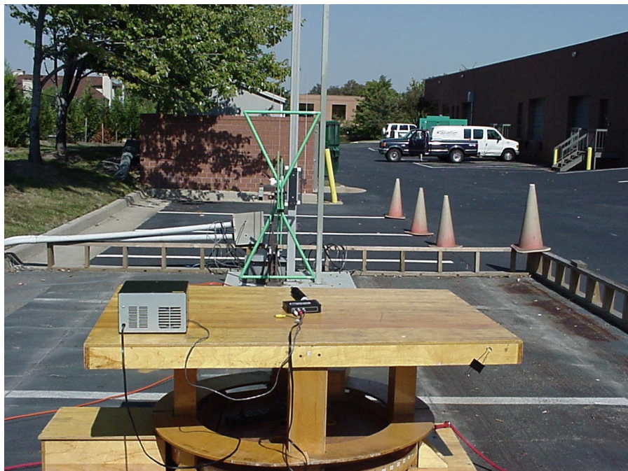
PHOTOGRAPH 2: RADIATED EMISSIONS REAR VIEW
