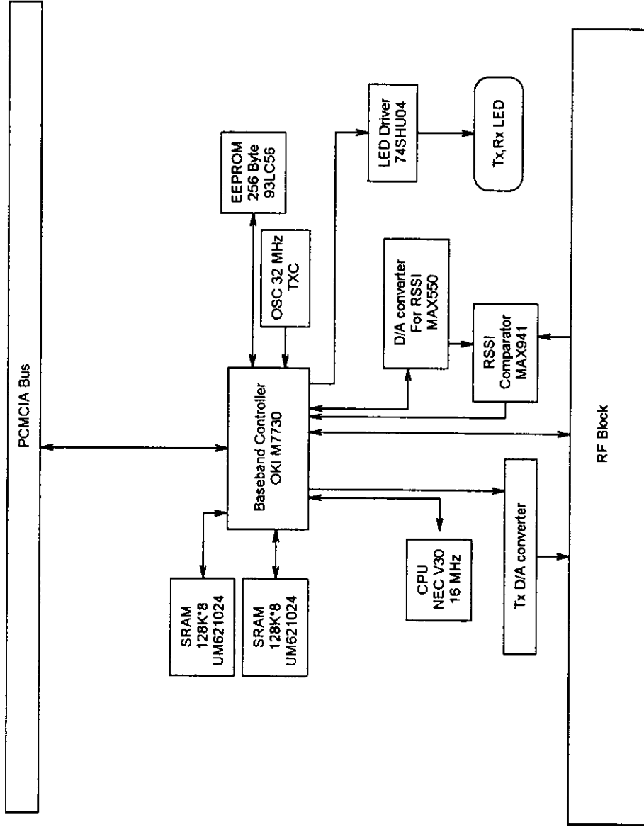
1 Mbps Plus PCMCIA Wireless LAN Adapter Function Block
