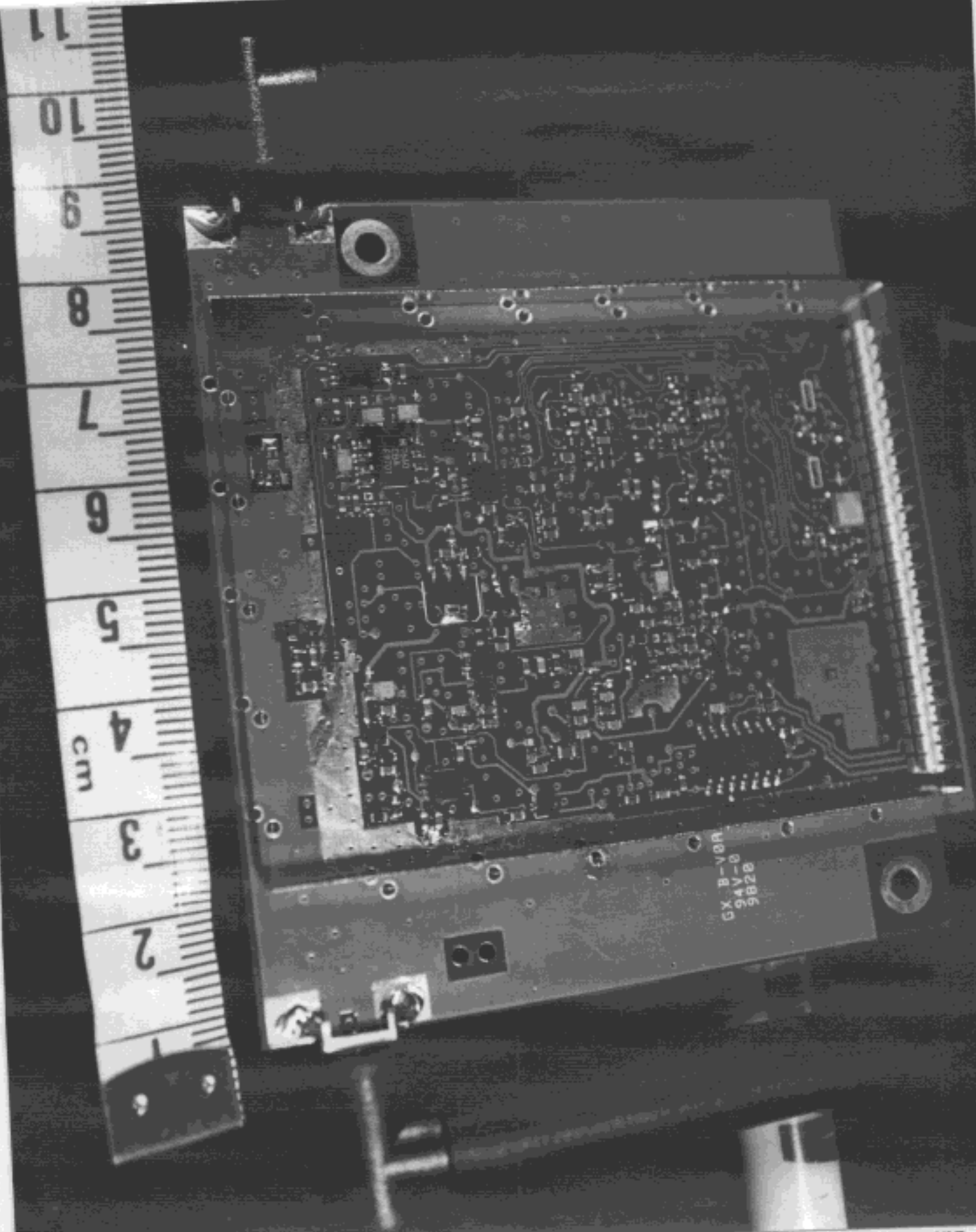
Back Side View of RF Module-2
