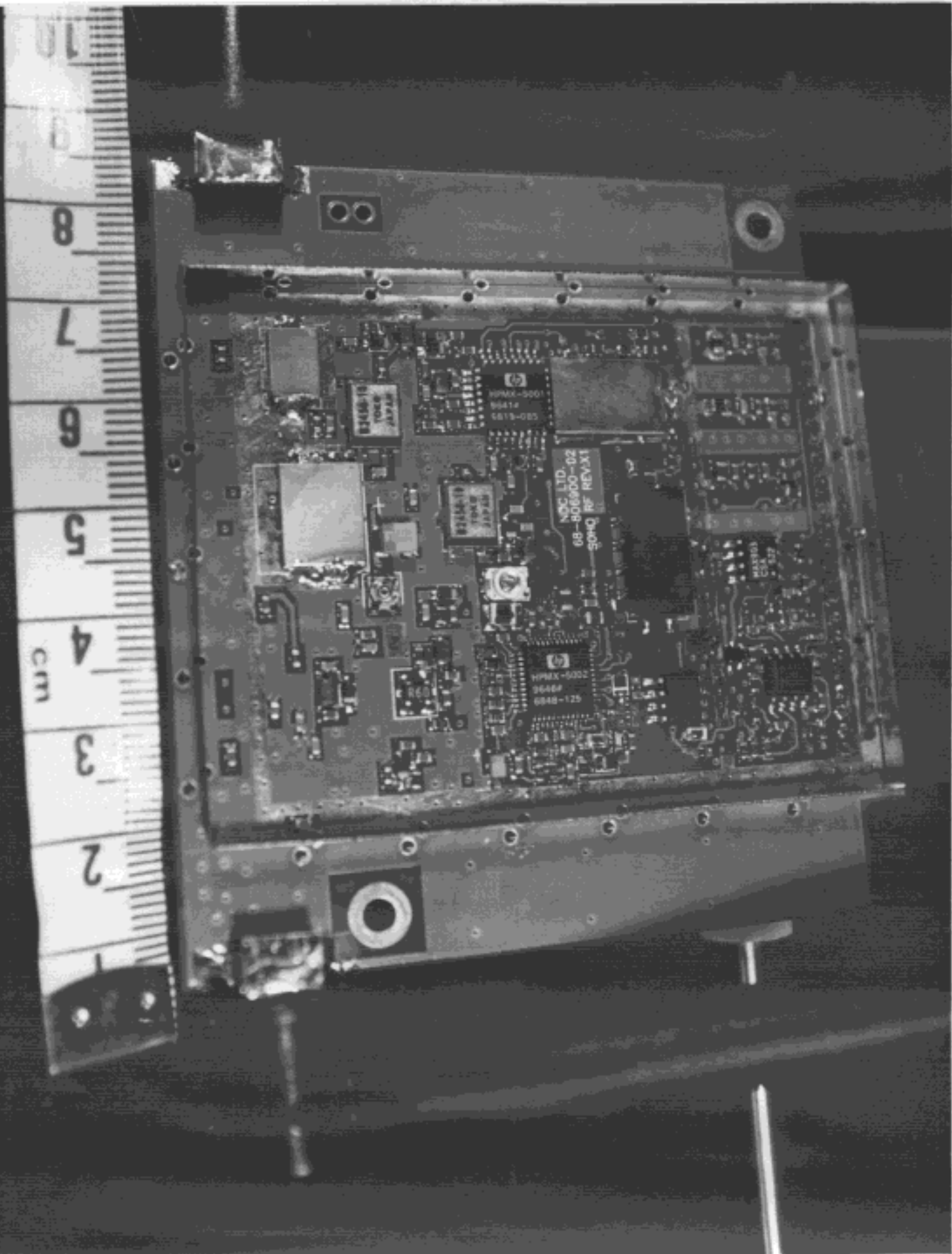
Top Side View of RF Module-2
