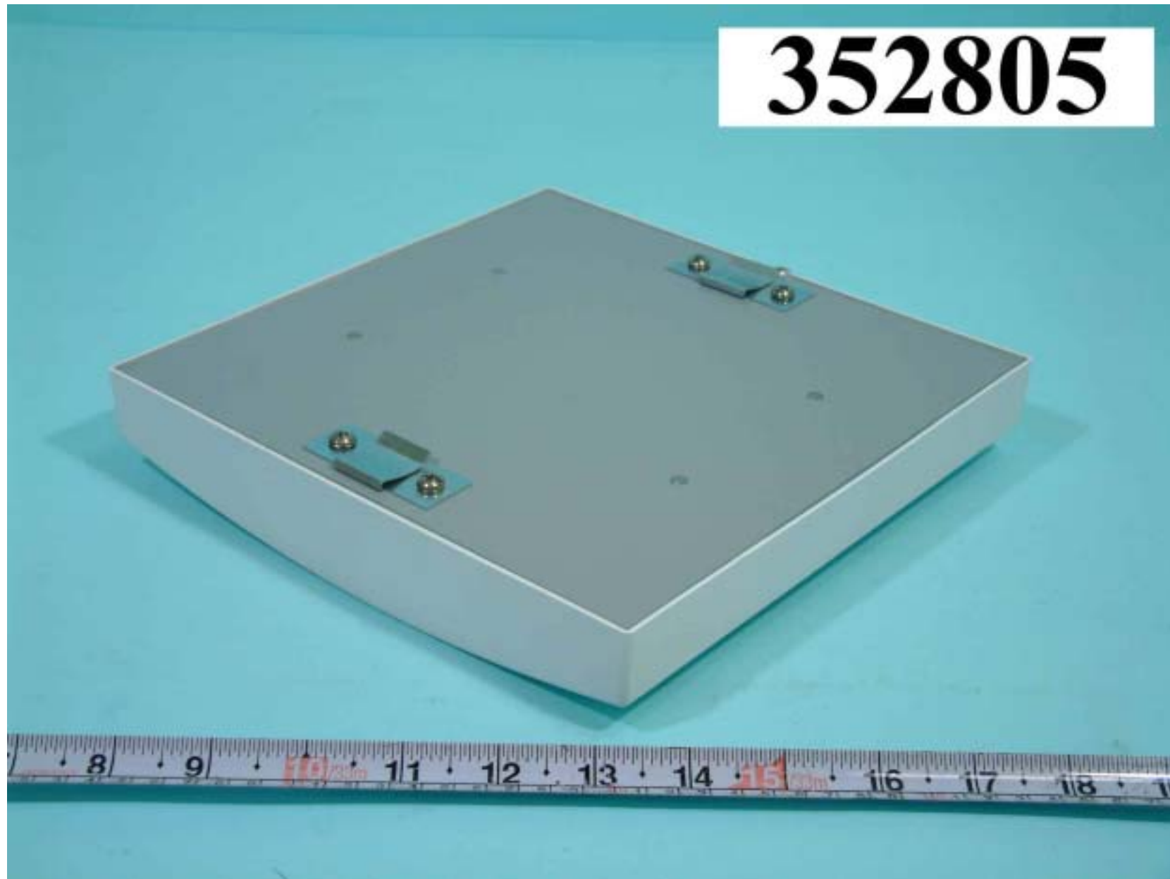
REAR SIDE OF ANTENNA (18dBi)
