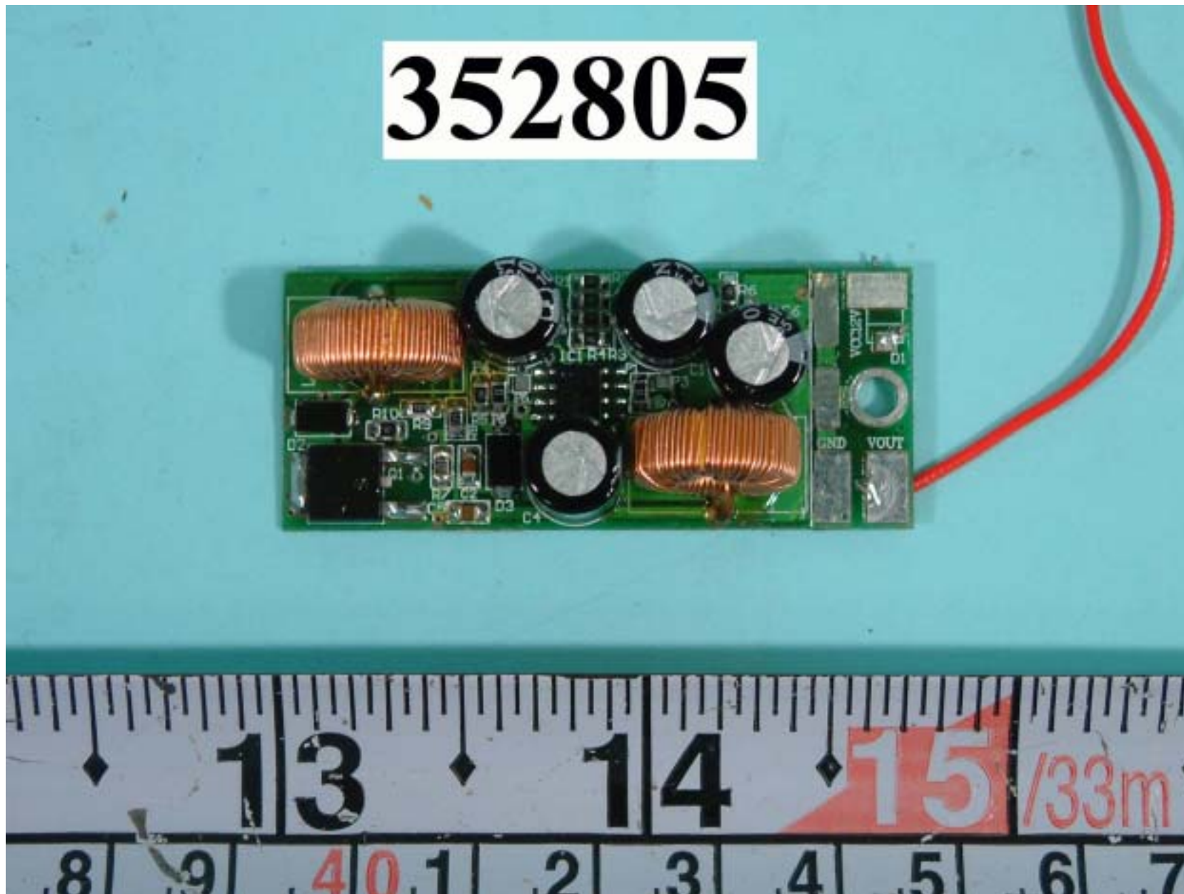
FRONT SIDE OF CIRCUIT BOARD OF EUT MAIN PART
