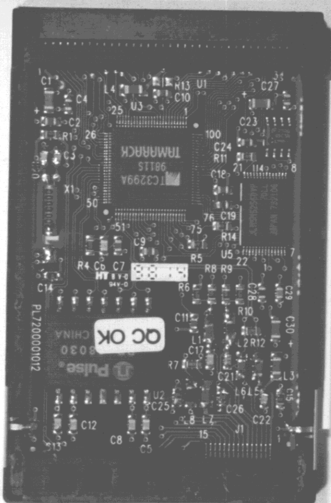
FCC ID: :IOUND5100ES01 Front side of main board
