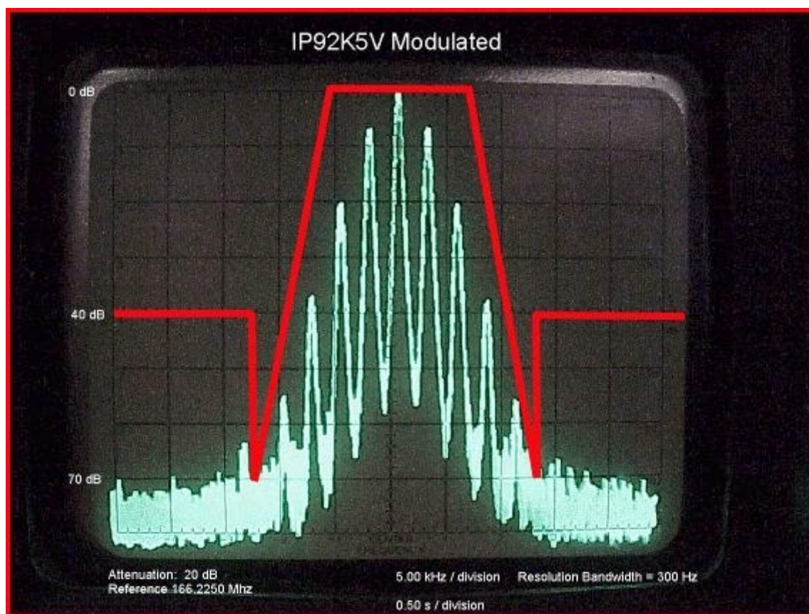
Figure 3 Modulated Bandwidth
